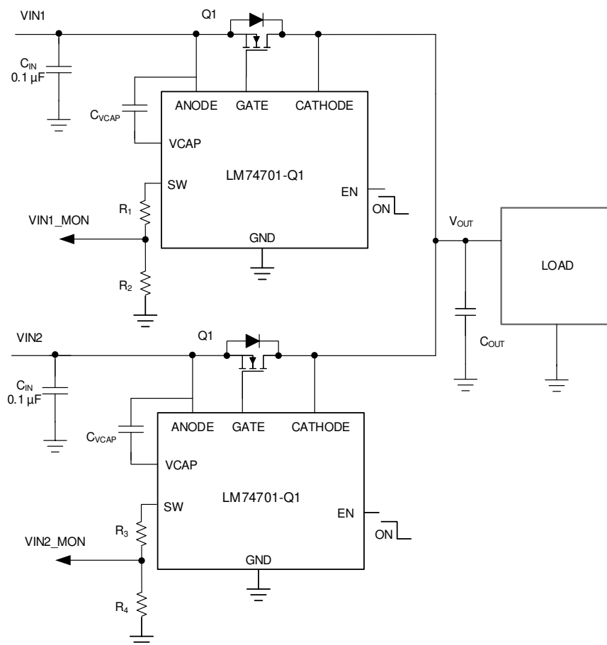
图 9-12. Typical OR-ing Application
