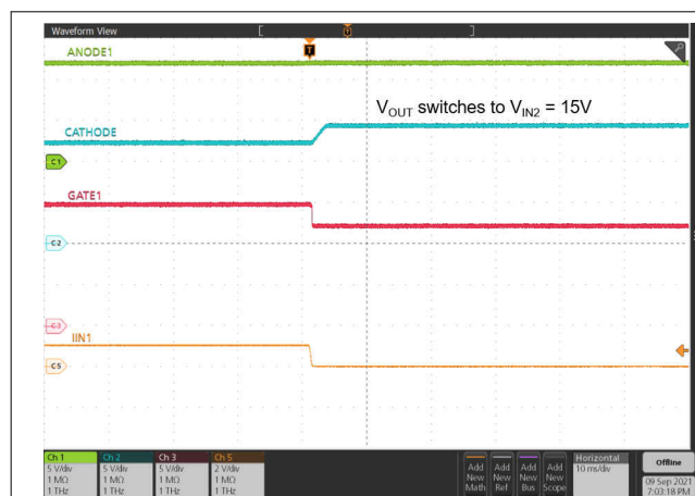
图 9-13. ORing V_{IN1} to V_{IN2} Switch Over
