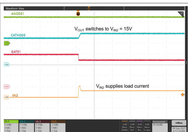
图 9-14. ORing V_{IN1} to V_{IN2} Switch Over
