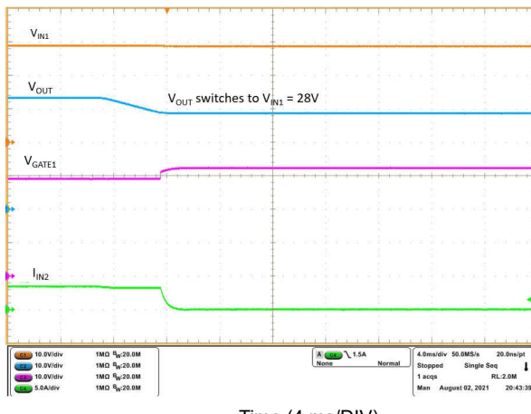
图 9-15. ORing V_{IN2} to V_{IN1} Switch Over
