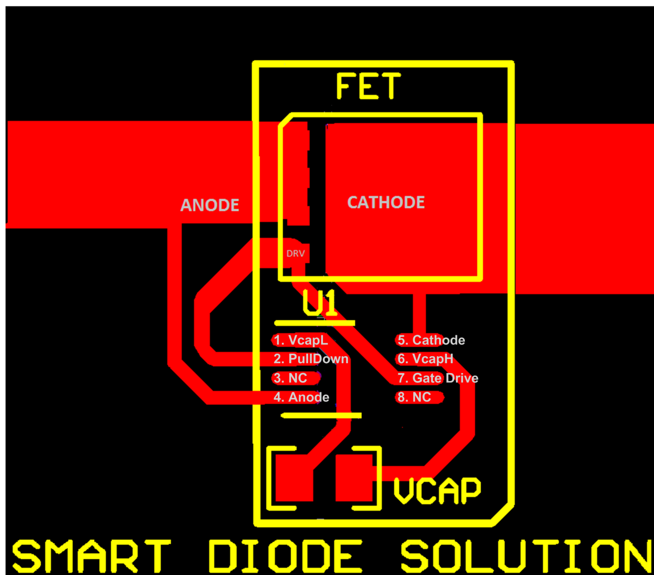
Figure 22. Layout Example
