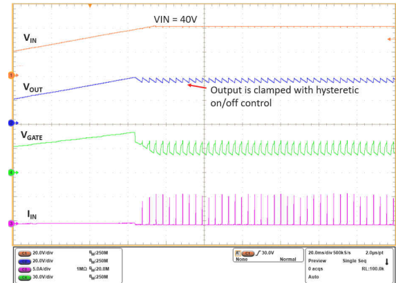
图 10-10. Overvoltage Clamp Response
