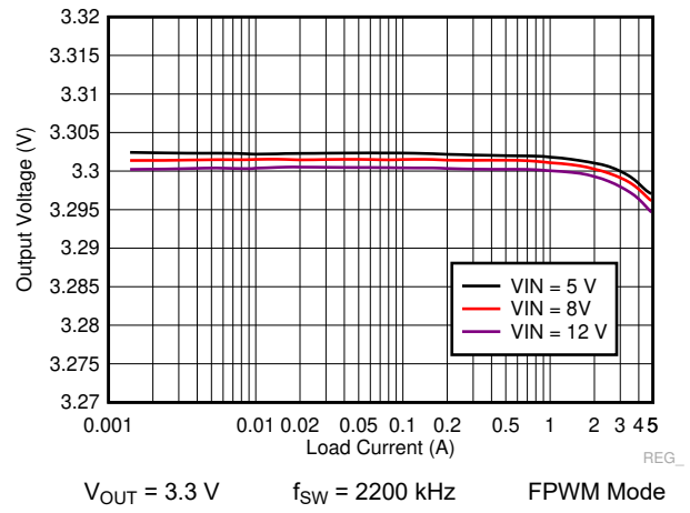
图 9-30. LM73605-Q1 Load and Line Regulation
