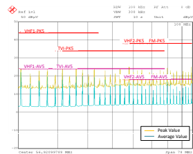
图 9-64. LM73606-Q1 Conducted EMI Result versus CISPR25 Limits - High Frequency
