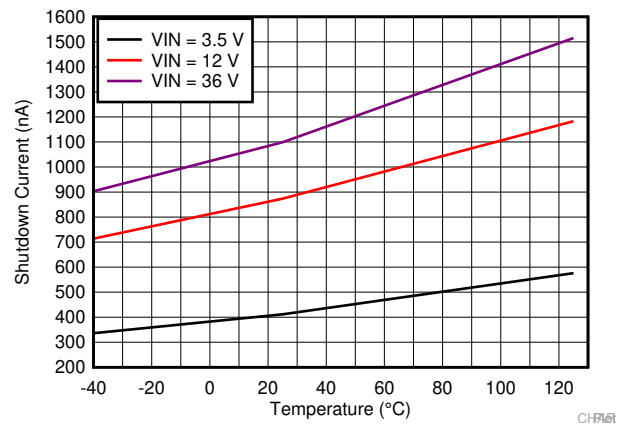
图 7-2. Shutdown Quiescent Current
