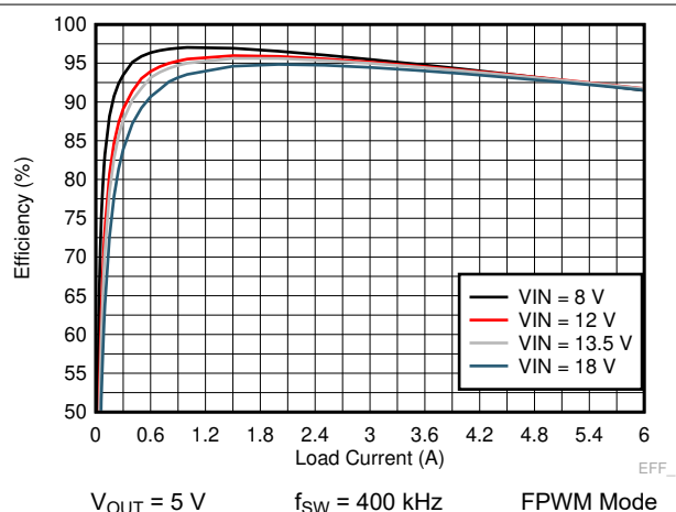
图 9-12. LM73606-Q1 Efficiency
