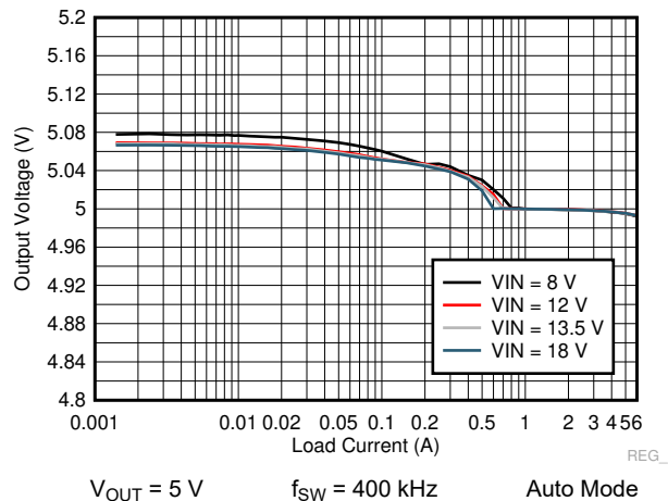
图 9-21. LM73606-Q1 Load and Line Regulation
