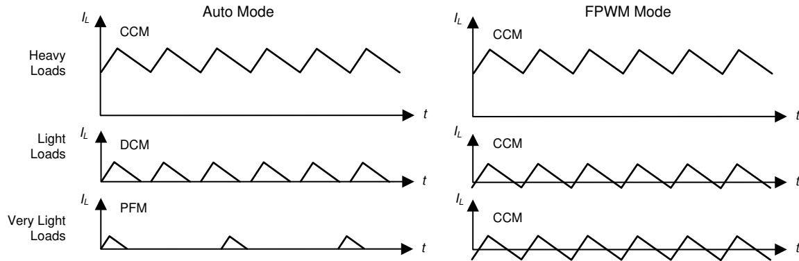
图 8-2. Inductor Current Waveforms at Auto Mode and FPWM Mode with Different Loads
