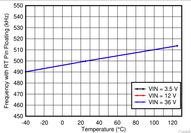
图 7-7. Switching Frequency with RT Pin Open Circuit
