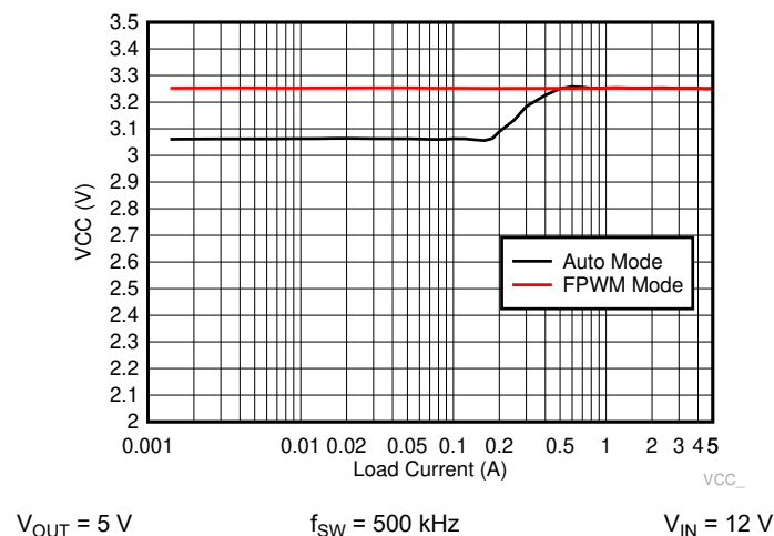
图 8-8. VCC Voltage versus Load Current
