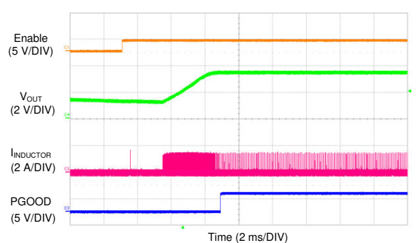
图 9-54. LM73606-Q1 Soft Start With 200-mA Load in Auto Mode
