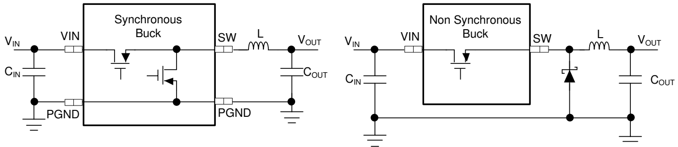
图 8-1. Simplified Synchronous versus Non-synchronous Buck Converters
