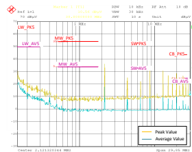
图 9-63. LM73606-Q1 Conducted EMI Result versus CISPR25 Limits - Low Frequency
