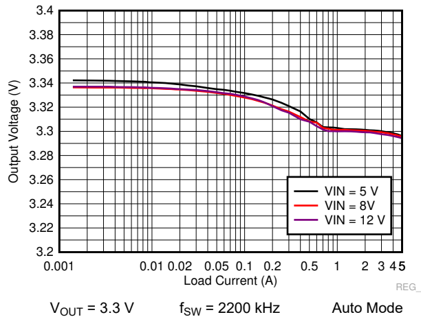
图 9-29. LM73605-Q1 Load and Line Regulation
