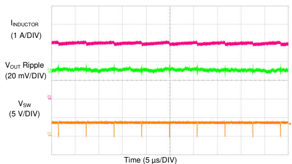
图 9-48. LM73606-Q1 Switching Waveform and V_{OUT} Ripple
