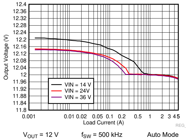
图 9-33. LM73605-Q1 Load and Line Regulation
