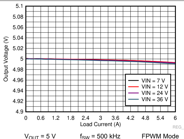
图 9-24. LM73606-Q1 Load and Line Regulation
