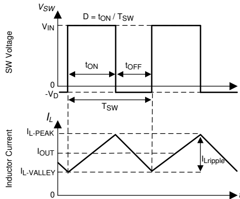
图 8-3. SW Voltage and Inductor Current Waveforms in CCM
