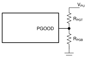
图 8-15. Divider for PGOOD Pullup Voltage
