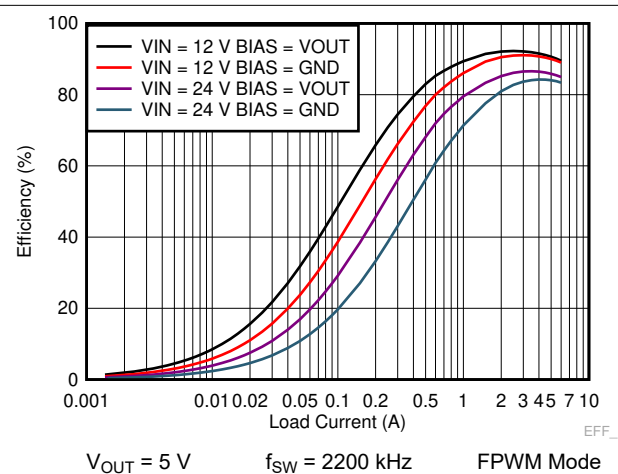
图 8-7. LM73606-Q1 Efficiency Comparison With Bias = V_{OUT} to Bias = GND in FPWM Mode
