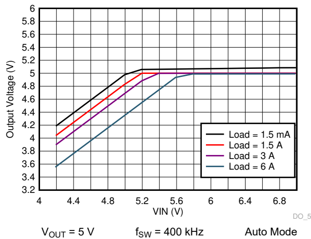
图 9-35. LM73606-Q1 Dropout Curve
