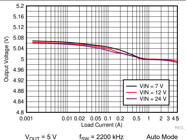
图 9-25. LM73605-Q1 Load and Line Regulation
