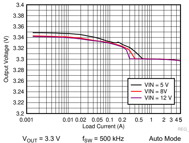
图 9-31. LM73605-Q1 Load and Line Regulation
