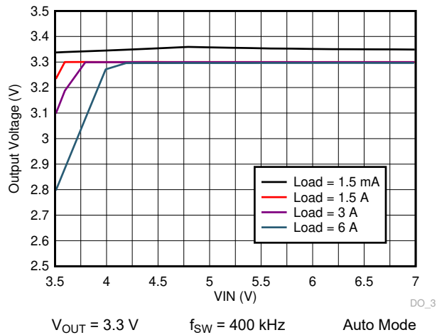
图 9-41. LM73606-Q1 Dropout Curve
