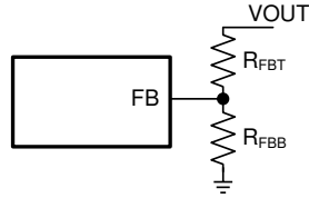
图 8-4. Output Voltage Setting by Resistor Divider
