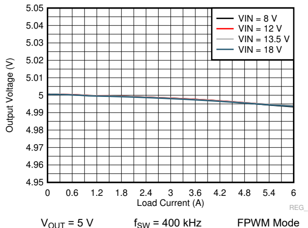
图 9-22. LM73606-Q1 Load and Line Regulation
