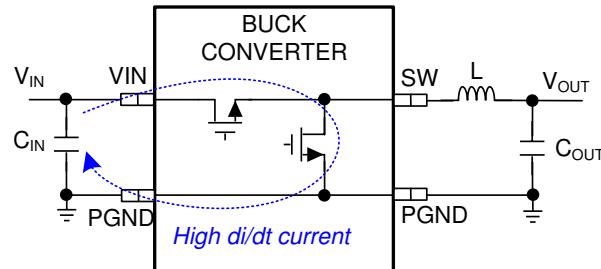
图 9-1. Pulsing Current Path of Buck Converter
