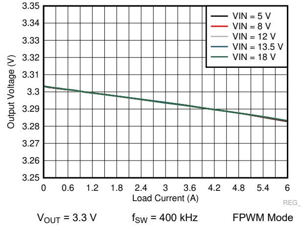
图 9-28. LM73606-Q1 Load and Line Regulation
