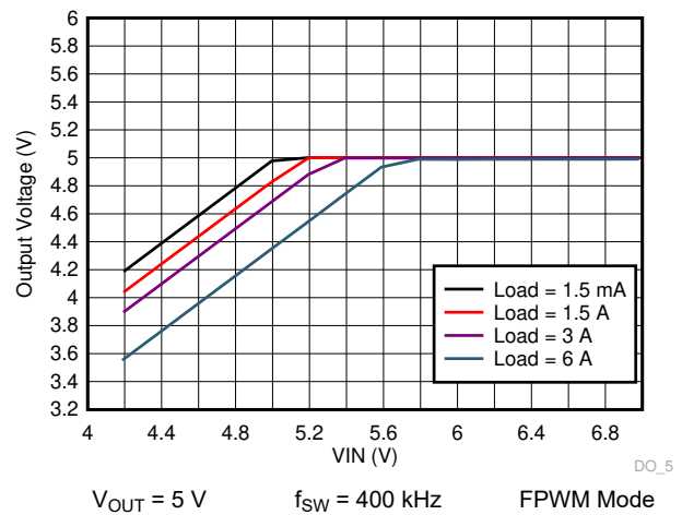
图 9-36. LM73606-Q1 Dropout Curve
