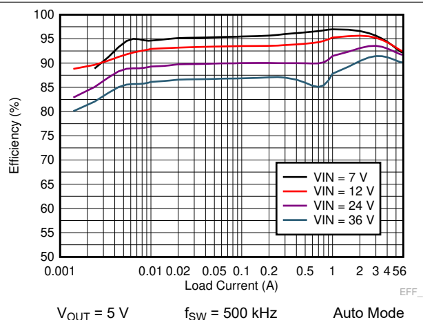
图 9-13. LM73606-Q1 Efficiency
