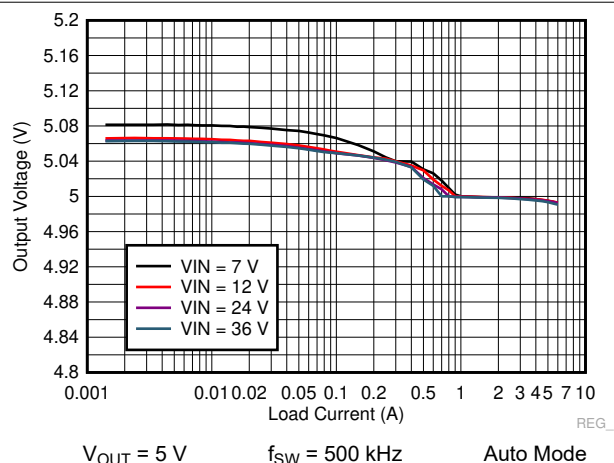
图 9-23. LM73606-Q1 Load and Line Regulation
