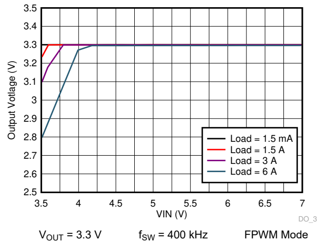
图 9-42. LM73606-Q1 Dropout Curve
