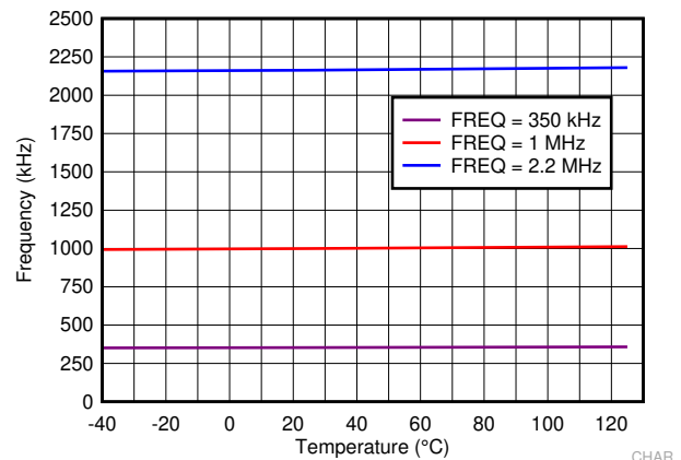
图 7-6. Switching Frequency Set by R_T Resistor
