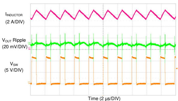
图 9-47. LM73606-Q1 Switching Waveform and V_{OUT} Ripple
