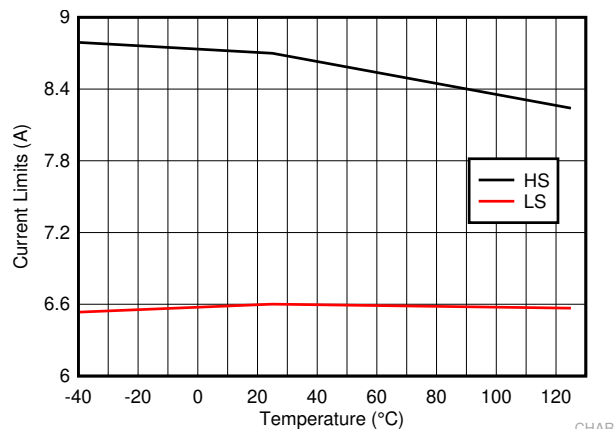
图 7-5. LM73605-Q1 High-Side and Low-Side Current Limit
