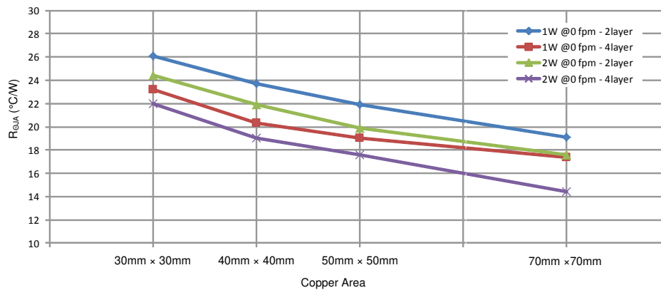
图 9-2. Measured R_{\theta JA} versus PCB Copper Area on 2-Layer Boards and 4-Layer Boards
