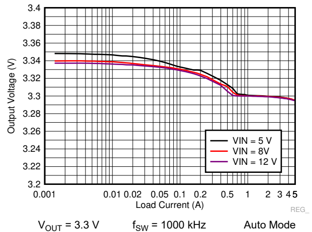
图 9-32. LM73605-Q1 Load and Line Regulation
