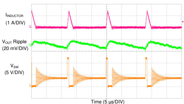
图 9-45. LM73606-Q1 Switching Waveform and V_{OUT} Ripple
