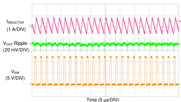
图 9-46. LM73606-Q1 Switching Waveform and V_{OUT} Ripple
