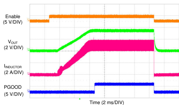
图 9-53. LM73606-Q1 Soft Start With 200-mA Load in FPWM Mode
