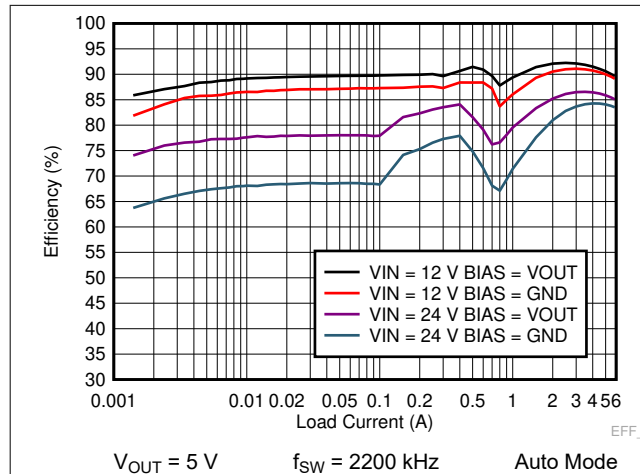
图 8-6. LM73606-Q1 Efficiency Comparison With Bias = V_{OUT} to Bias = GND in Auto Mode
