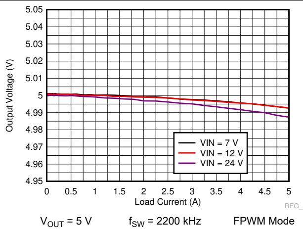
图 9-26. LM73605-Q1 Load and Line Regulation
