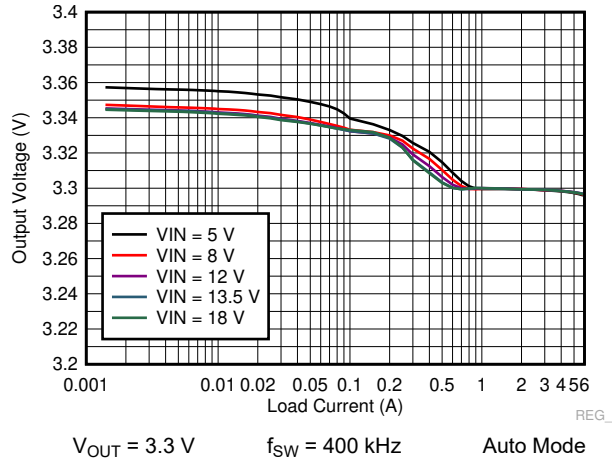
图 9-27. LM73606-Q1 Load and Line Regulation
