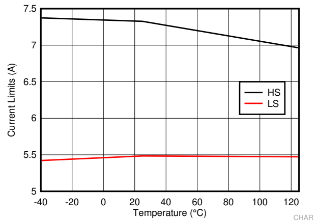
图 7-4. LM73605-Q1 High-Side and Low-Side Current Limits
