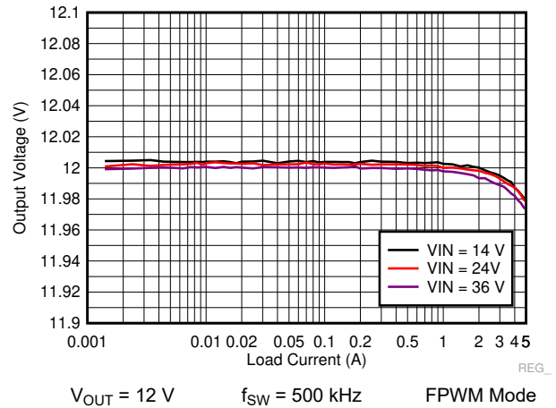
图 9-34. LM73605-Q1 Load and Line Regulation
