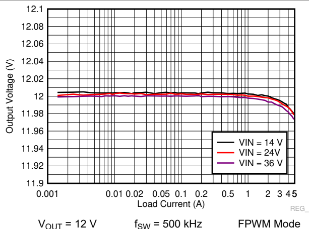
图 9-34. LM73605-Q1 Load and Line Regulation
