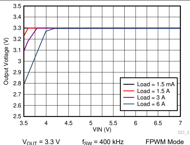
图 9-42. LM73606-Q1 Dropout Curve
