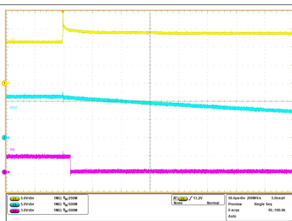
图 8-5. Overvoltage protection
