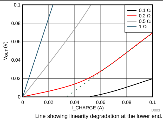
Figure 30. Low-End Transfer Function for Various R_{\text{SENSE}}
