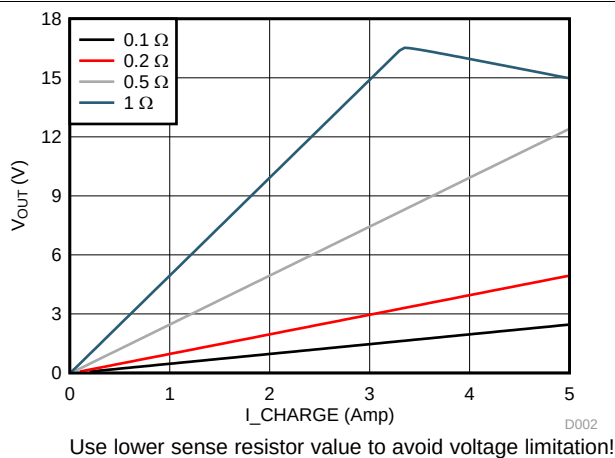
Figure 29. Current Sense Transfer Function for Various R_{\text{SENSE}} Values
