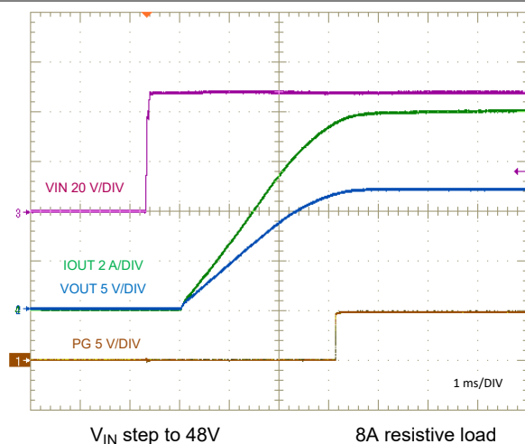
图 8-24. Start-Up Characteristic
