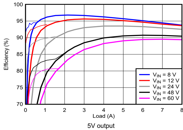
图 6-1. Efficiency versus I_{OUT}
