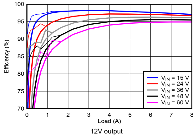
图 6-3. Efficiency versus I_{OUT}
