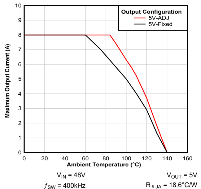
图 8-5. Maximum Output Current versus Ambient Temperature
