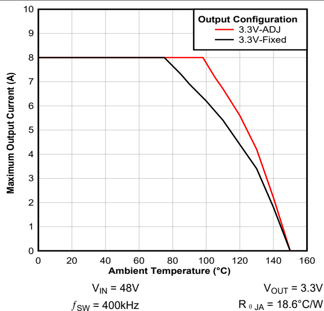
图 8-4. Maximum Output Current versus Ambient Temperature
