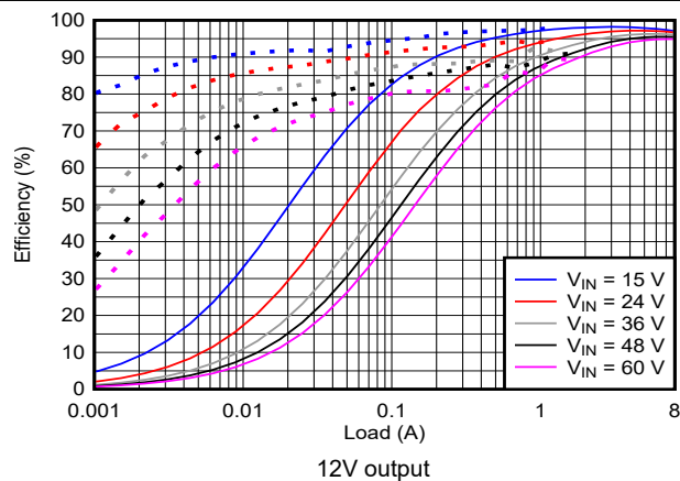
图 8-21. Efficiency versus I_{OUT} , Log Scale
