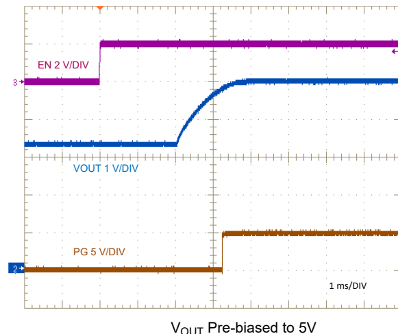
图 8-16. EN Start-Up Pre-bias Characteristic
