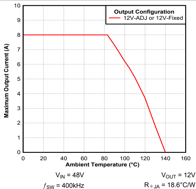
图 8-7. Maximum Output Current versus Ambient Temperature
