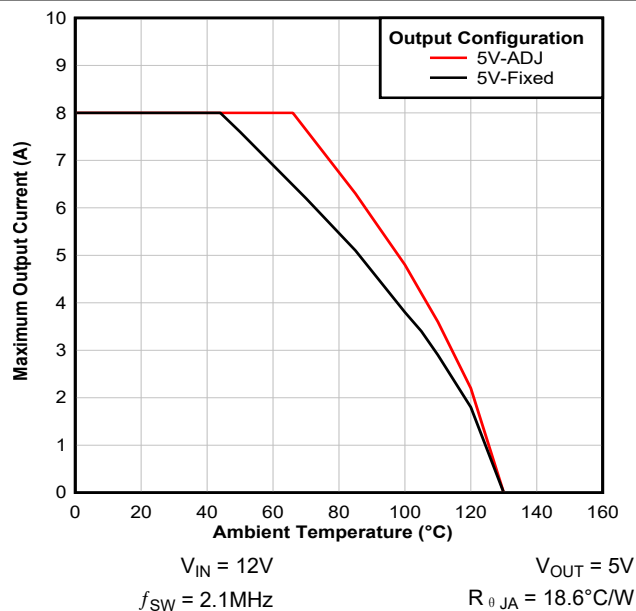
图 8-6. Maximum Output Current versus Ambient Temperature
