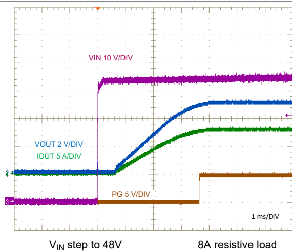
图 8-13. Start-Up Characteristic
