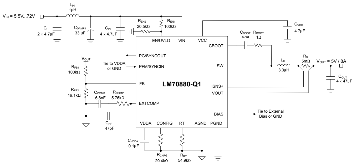
图 8-8. Application Circuit 1 With LM70880-Q1 Buck Regulator at 400kHz
