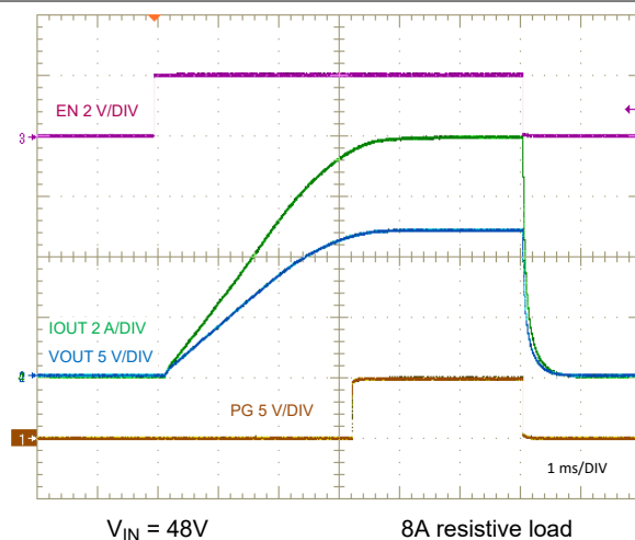
图 8-25. EN Start-Up Characteristic
