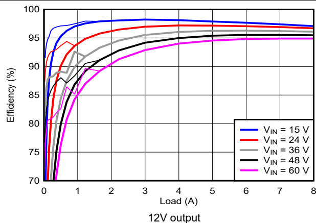
图 8-20. Efficiency versus I_{OUT}
