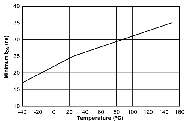
图 6-10. Minimum On-Time vs Temperature
