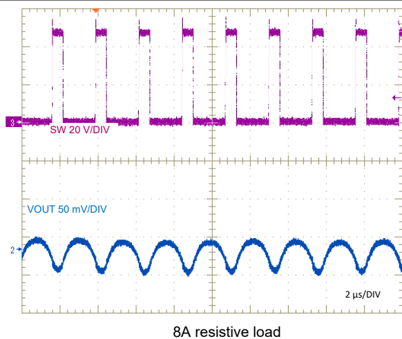
图 8-22. Full load Switching
