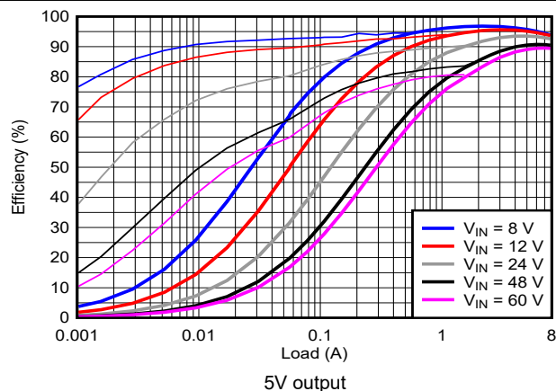
图 8-10. Efficiency versus I_{OUT} , Log Scale
