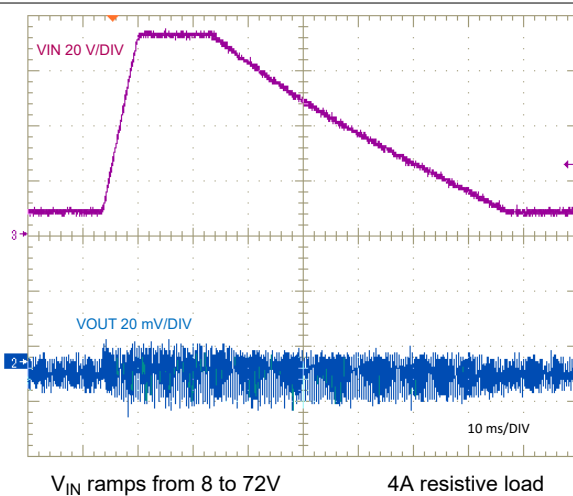
图 8-14. Line Transient Response to V_{IN} = 72V
