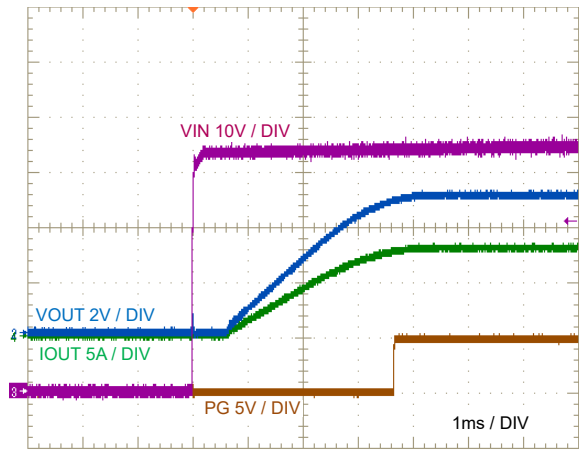
V_{IN} 降压至 48V I_{OUT} = 8A ( 电阻负载 ) FPWM V_{OUT} = 5V F_{SW} = 400kHz
