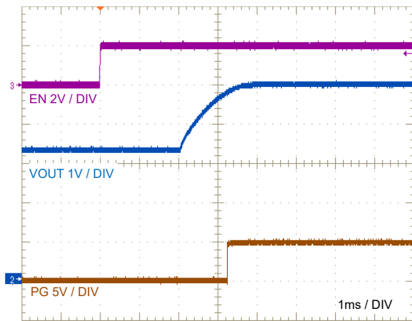
V_{IN} = 48V I_{OUT} = 8A ( 电阻负载 ) FPWM V_{OUT} = 预偏置为 5V F_{SW} = 400kHz
