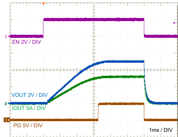
V_{IN} = 48V I_{OUT} = 8A ( 电阻负载 ) FPWM V_{OUT} = 5V F_{SW} = 400kHz
