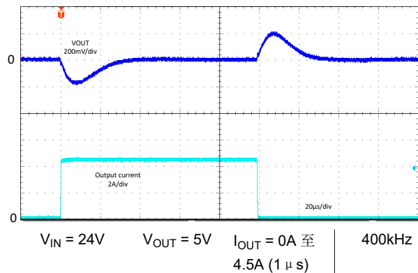
图 8-85. 负载瞬态 — LM6x645 — FPWM
