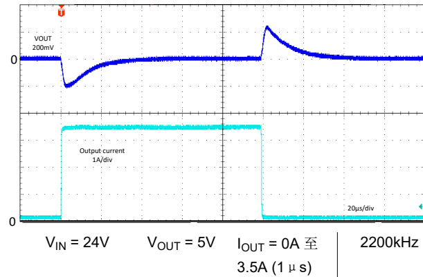
图 8-83. 负载瞬态 — LM6x635 — FPWM
