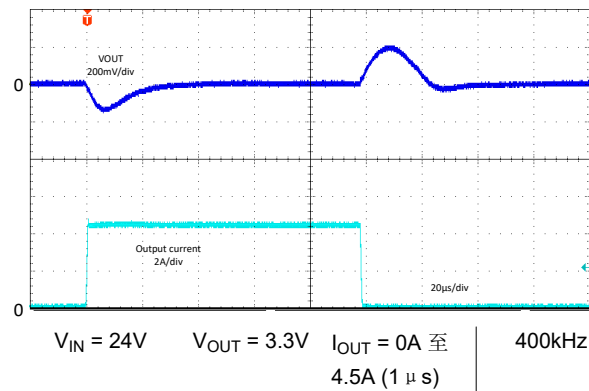
图 8-86. 负载瞬态 — LM6x645 — FPWM
