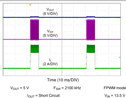
图 10-22. LM62440-Q1 Short Circuit Performance
