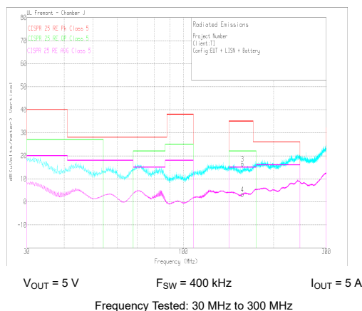
图 9-28. Radiated EMI Bicon Vertical versus CISPR25 Limits
