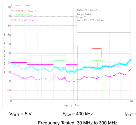
图 9-28. Radiated EMI Bicon Vertical versus CISPR25 Limits
