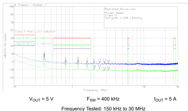
图 9-27. Radiated EMI Rod versus CISPR25 Limits
