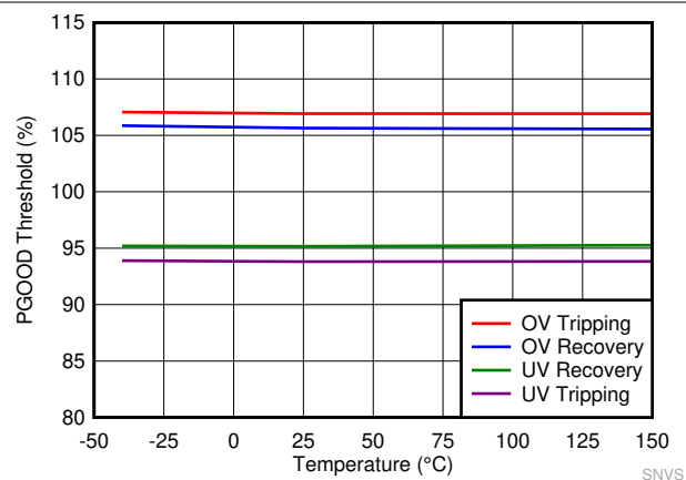
图 7-8. PGOOD Thresholds
