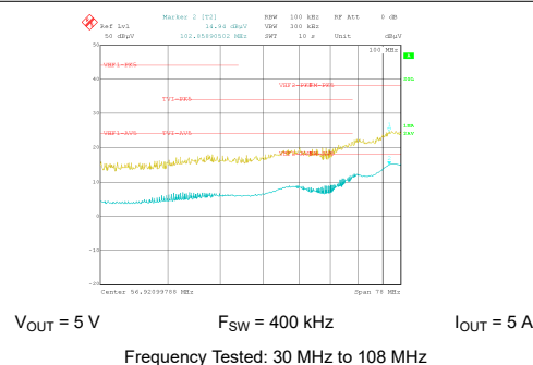
图 9-26. Conducted EMI versus CISPR25 Limits (Yellow: Peak Signal, Blue: Average Signal)
