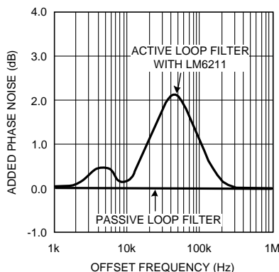
Figure 40. Effect of LM6211 on Phase Noise of PLL
