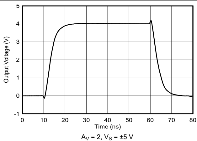
图 5-31. Large-Signal Pulse Response
