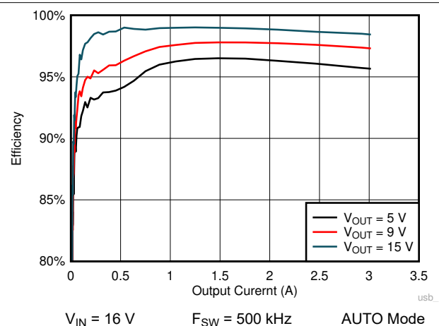
图 9-67. LM61460 Efficiency
