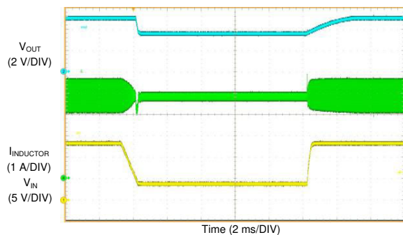
图 9-43. LM61460 Short Circuit Recovery
