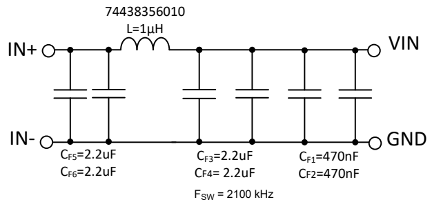
图 9-64. Recommended Input EMI Filter
