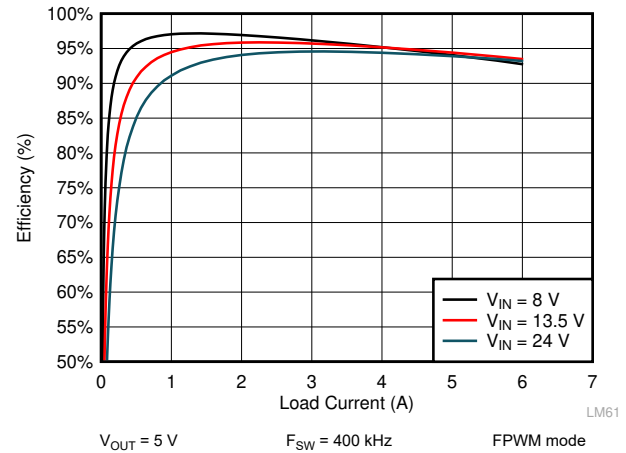
图 9-12. LM61460 Efficiency
