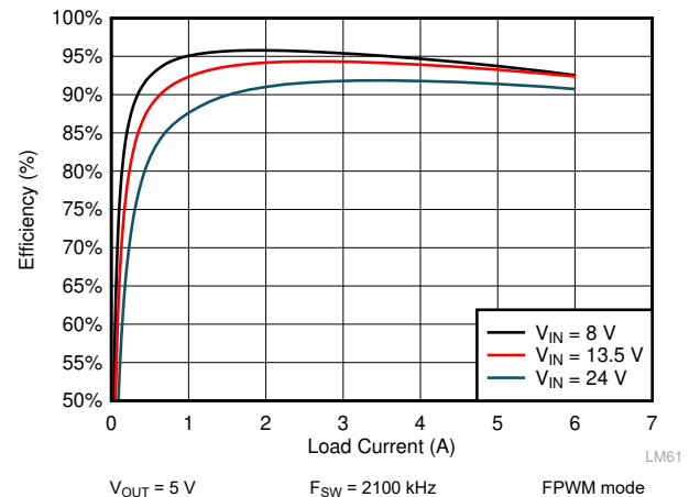
图 9-16. LM61460 Efficiency
