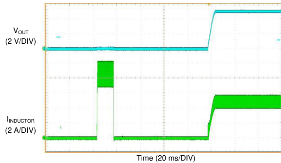
图 9-41. LM61460 Start-up with 3.25-A
