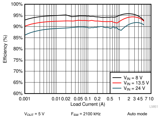
图 9-15. LM61460 Efficiency
