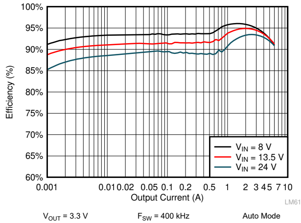
图 9-5. LM61460 Efficiency
