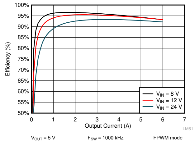
图 9-14. LM61460 Efficiency
