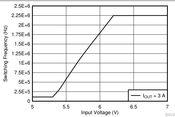
图 10-24. LM61440-Q1 Frequency Dropout Curve
