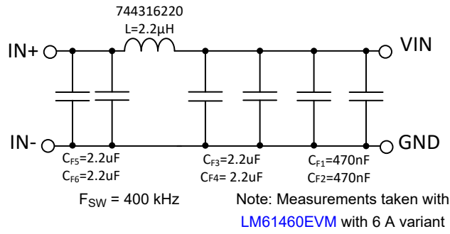
图 10-41. Recommended Input EMI Filter
