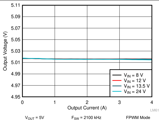
图 9-15. LM61440 Load and Line Regulation
