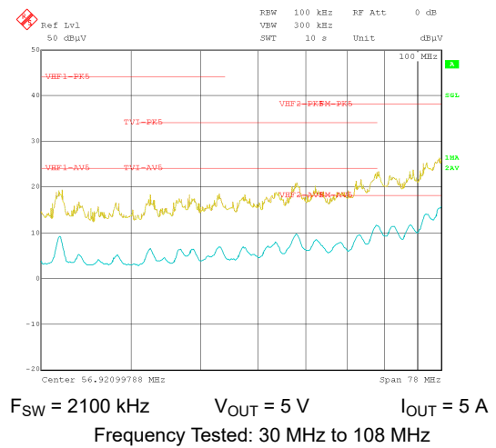
图 9-42. Conducted EMI versus CISPR25 Limits (Yellow: Peak Signal, Blue: Average Signal)
