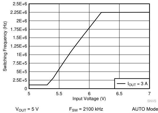
图 9-23. LM61440 Frequency Dropout Curve
