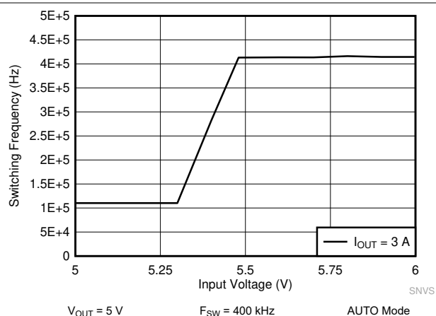
图 9-22. LM61440 Frequency Dropout Curve
