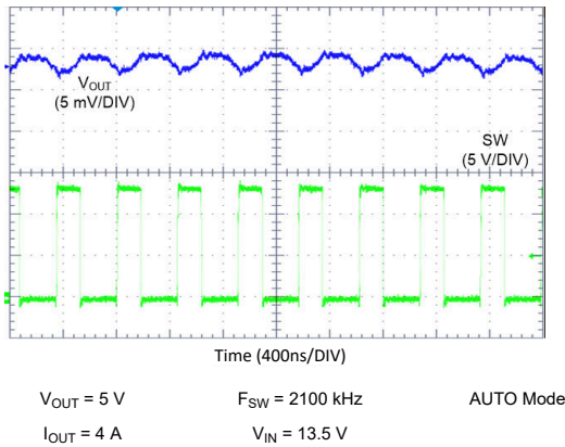
图 9-25. LM61440 Switching Waveform and V_{OUT} Ripple
