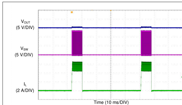
图 8-13. Inductor Current Bursts During Hiccup
