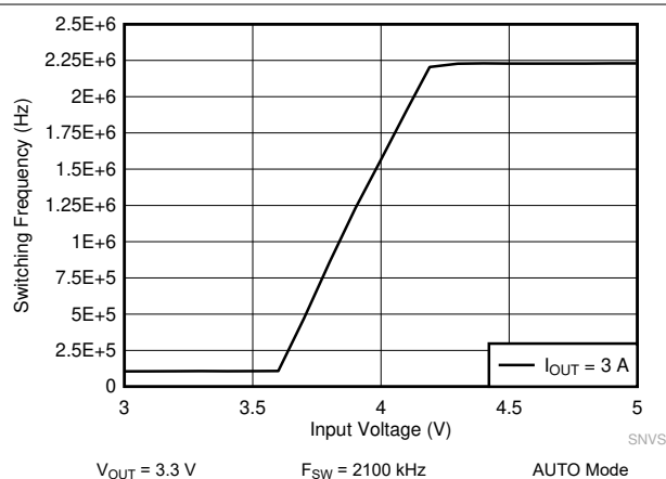
图 9-21. LM61440 Frequency Dropout Curve
