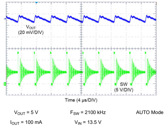
图 9-24. LM61440 Switching Waveform and V_{OUT} Ripple
