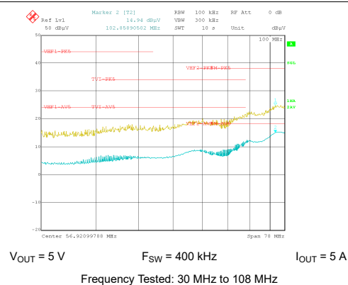
图 9-34. Conducted EMI versus CISPR25 Limits (Yellow: Peak Signal, Blue: Average Signal)
