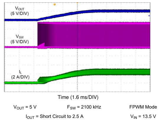
图 9-28. LM61440 Short Circuit Recovery
