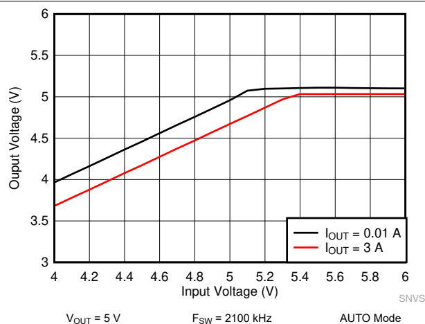
图 9-19. LM61440 Dropout Curve
