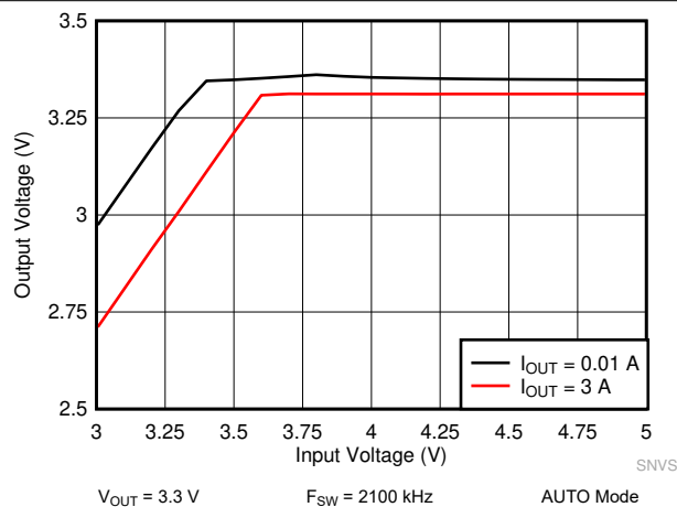
图 9-17. LM61440 Dropout Curve
