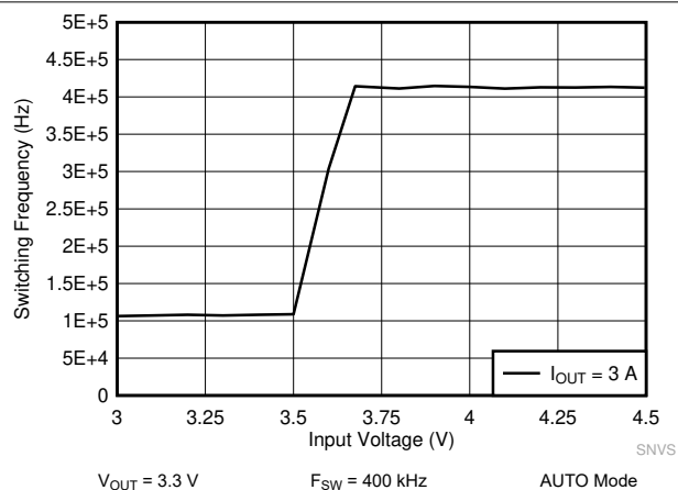
图 9-20. LM61440 Frequency Dropout Curve
