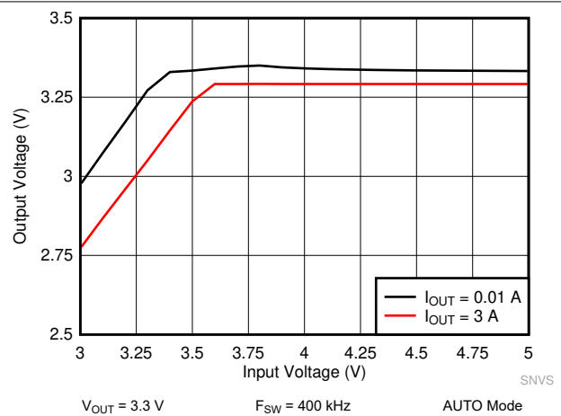
图 9-16. LM61440 Dropout Curve
