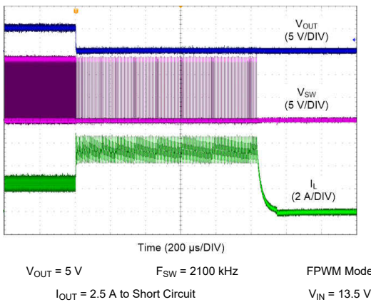
图 9-27. LM61440 Short Circuit Protection
