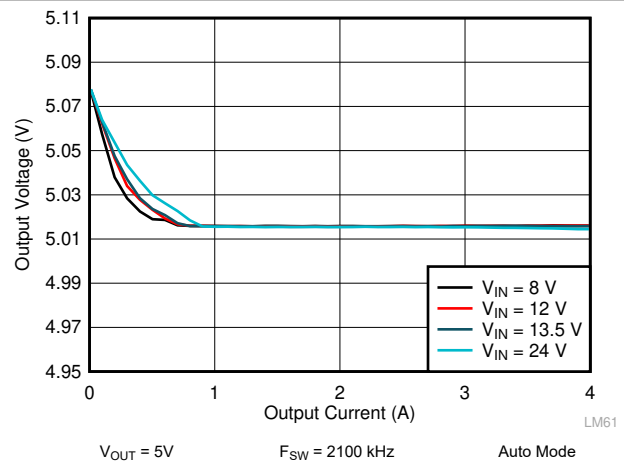
图 9-14. LM61440 Load and Line Regulation
