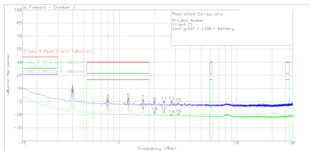
图 9-35. Radiated EMI Rod versus CISPR25 Limits
