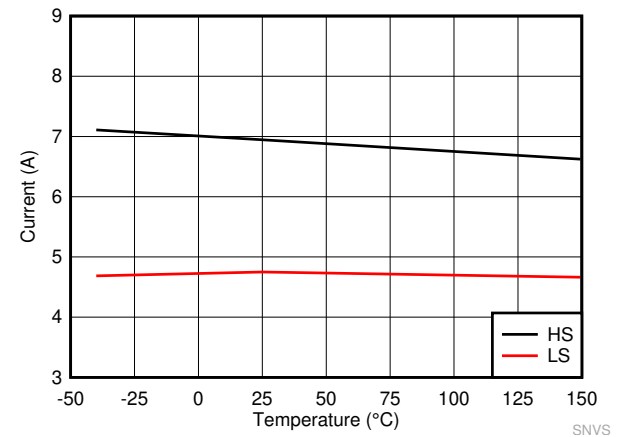
图 7-4. LM61440 High-side and Low-side Current Limits
