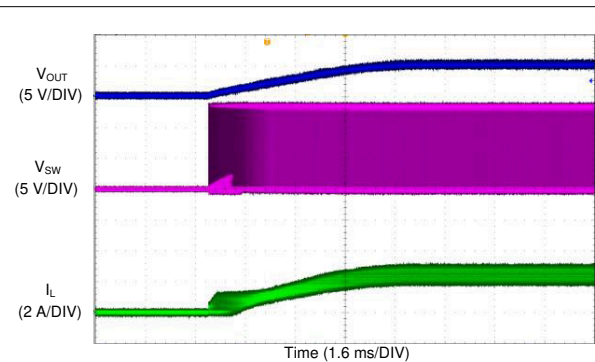
图 8-14. Short Circuit Recovery
