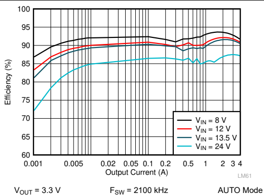
图 9-5. LM61440 Efficiency
