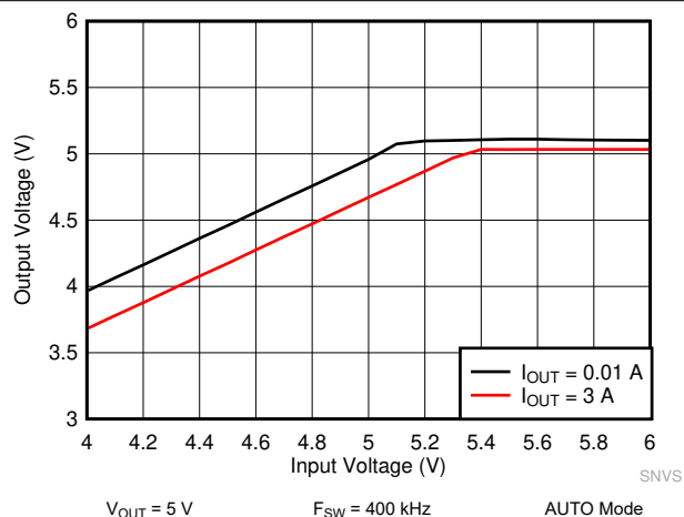
图 9-18. LM61440 Dropout Curve
