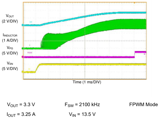
图 9-26. LM61440 Start-up with 3.25-A
