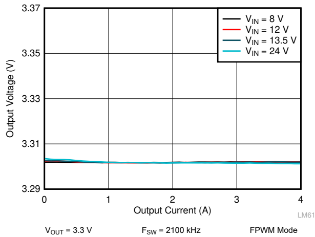
图 9-11. LM61440 Load and Line Regulation
