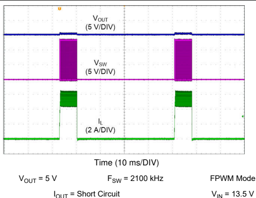
图 9-29. LM61440 Short Circuit Performance
