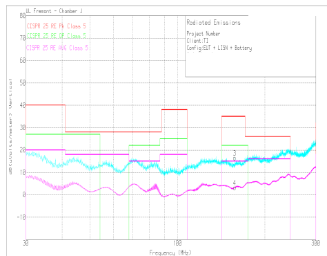
图 9-36. Radiated EMI Bicon Vertical versus CISPR25 Limits
