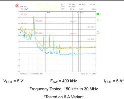
图 9-33. Conducted EMI versus CISPR25 Limits (Yellow: Peak Signal, Blue: Average Signal)
