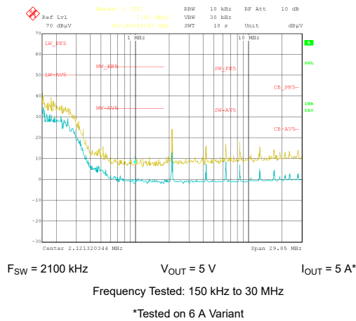
图 9-41. Conducted EMI versus CISPR25 Limits (Yellow: Peak Signal, Blue: Average Signal)
