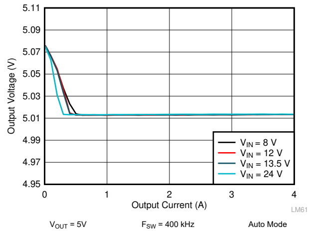
图 9-12. LM61440 Load and Line Regulation
