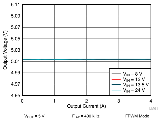
图 9-13. LM61440 Load and Line Regulation
