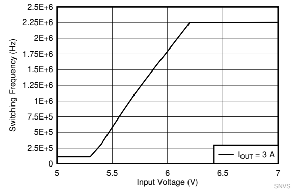
图 9-24. LM61435-Q1 Frequency Dropout Curve
