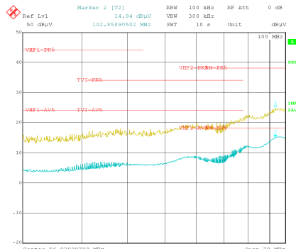
图 9-35. Conducted EMI versus CISPR25 Limits (Yellow: Peak Signal, Blue: Average Signal)
