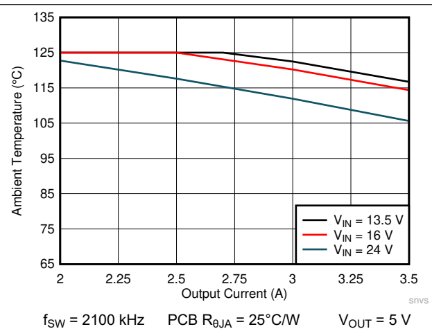
图 9-3. Maximum Ambient Temperature versus Output Current
