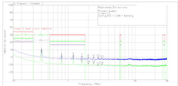
图 9-36. Radiated EMI Rod versus CISPR25 Limits
