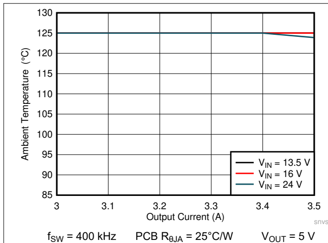
图 9-2. Maximum Ambient Temperature versus Output Current
