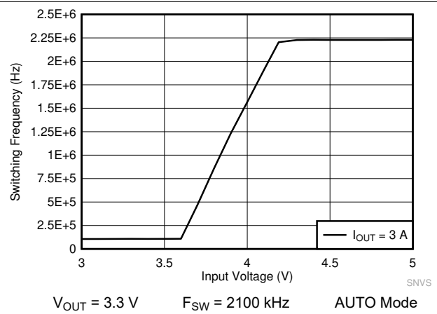
图 9-22. LM61435-Q1 Frequency Dropout Curve
