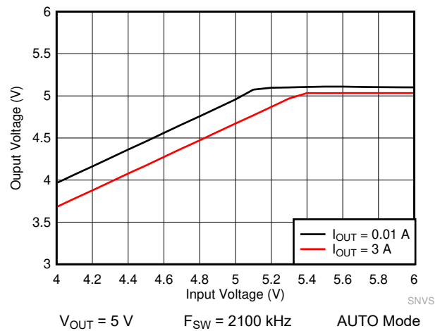
图 9-20. LM61435-Q1 Dropout Curve
