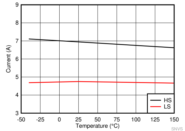
图 7-4. LM61435-Q1 High-side and Low-side Current Limits
