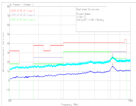
图 9-37. Radiated EMI Bicon Vertical versus CISPR25 Limits
