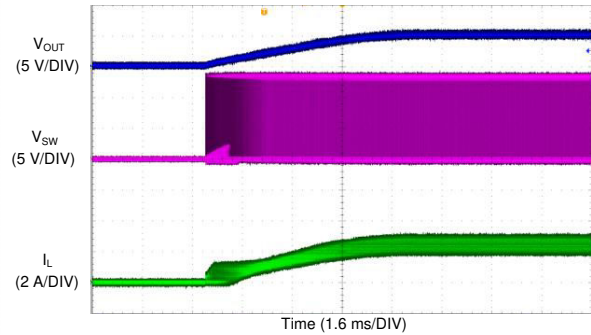
图 8-13. Short Circuit Recovery
