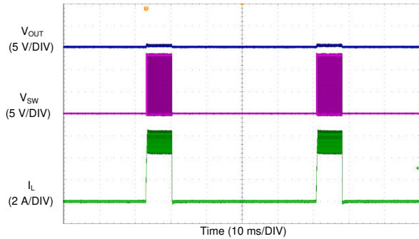
图 8-12. Inductor Current Bursts During Hiccup
