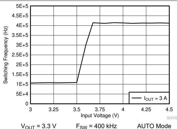
图 9-21. LM61435-Q1 Frequency Dropout Curve
