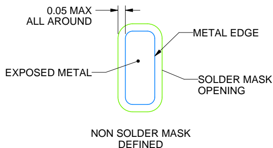
NON SOLDER MASK DEFINED SOLDER MASK DETAIL
