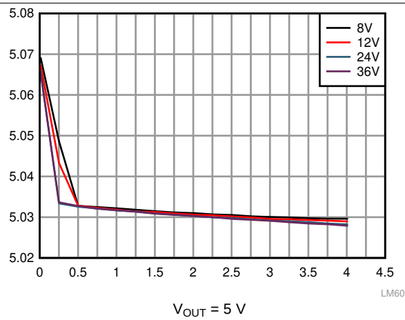
图 13. Line and Load Regulation
