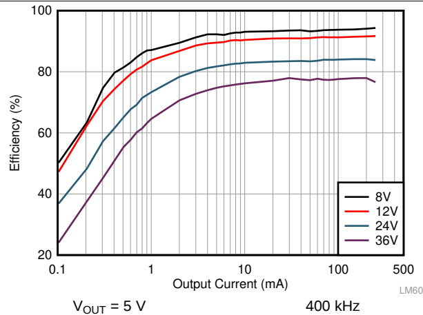
图 11. Low-Load Efficiency
