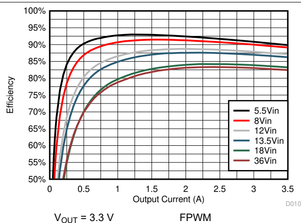
图 9-21. Efficiency
