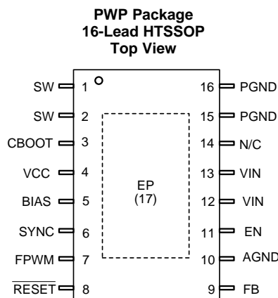
Pin Functions
