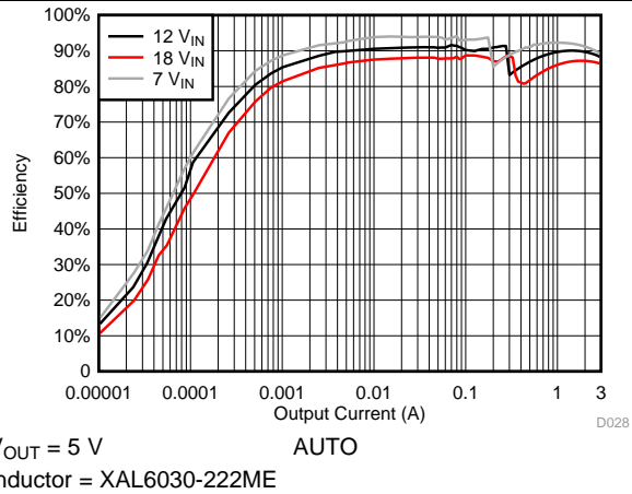
Figure 21. Efficiency
