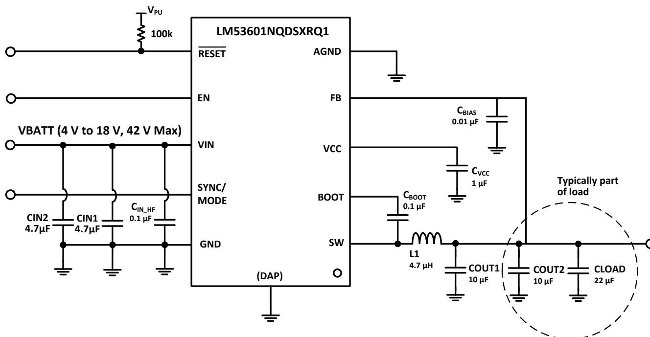
图 9-12. Typical LM53601NQDSXRQ1 Application Schematic
