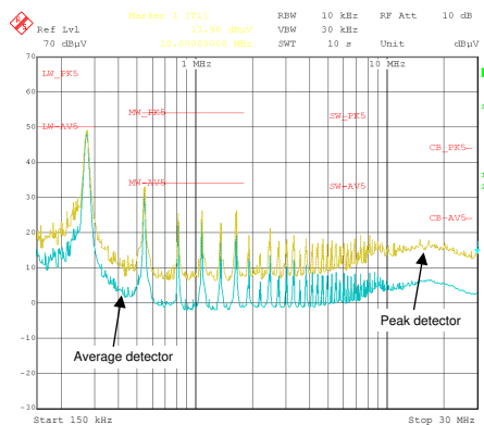
图 9-6. CISPR 25 Class 5 Conducted EMI Plot
