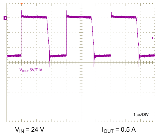
图 9-5. Flyback Diode Voltage
