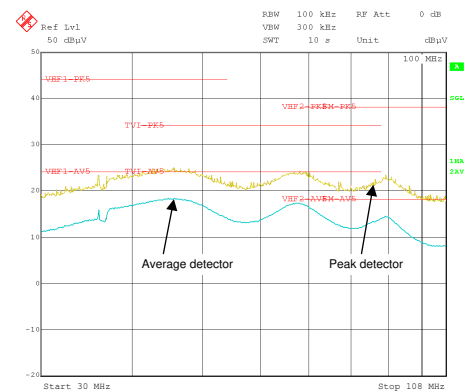
图 9-7. CISPR 25 Class 5 Conducted EMI Plot
