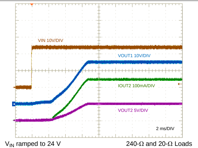
图 53. Start-Up Characteristic
