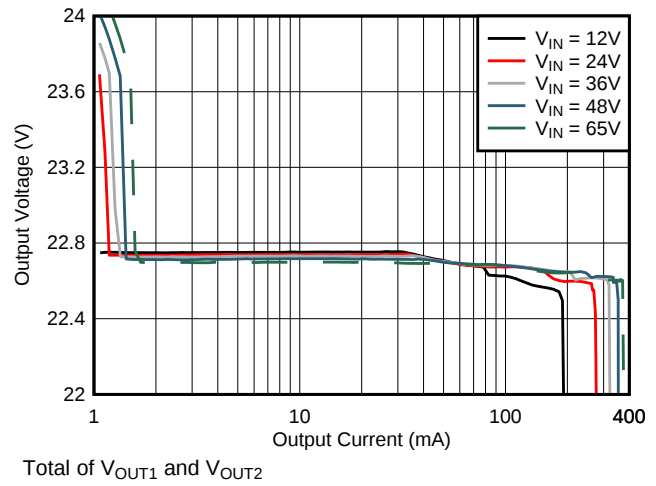
图 42. Load Regulation (Log Scale)
