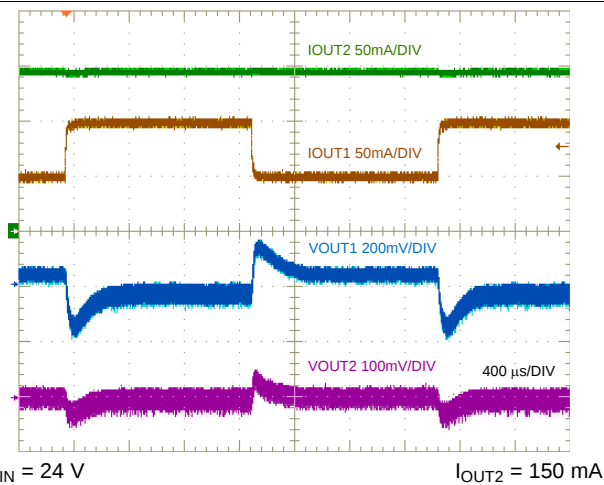
图 60. Output 1 Load Transient, 50 mA to 100 mA
