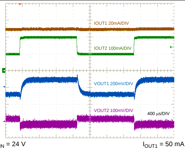
图 61. Output 2 Load Transient, 100 mA to 200 mA
