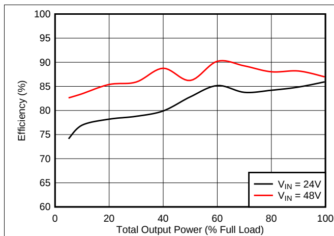
图 52. Efficiency
