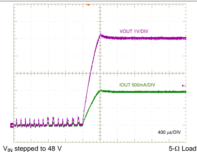
图 31. Short Circuit Recovery
