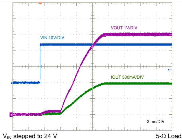
图 29. Start-up Characteristic
