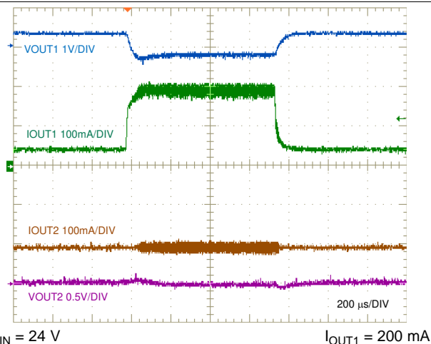
图 49. Output 1 Load Transient, 50 mA to 200 mA
