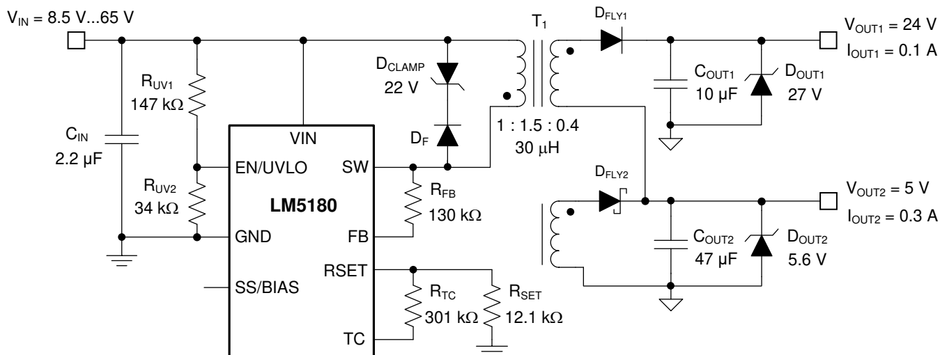
图 51. Schematic for Design 3 With V_{IN(nom)} = 24 V, V_{OUT1} = 24 V, V_{OUT2} = 5 V
