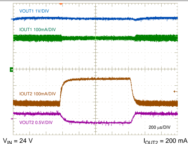
图 50. Output 2 Load Transient, 50 mA to 200 mA
