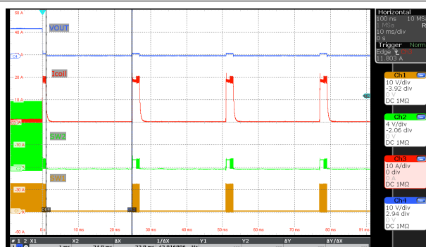
图 9-17. SCP ( V_{(VIN)} = 12V , V_{(VOUT)} = 12V , I_O = 短路, MODE = VCC2 )
