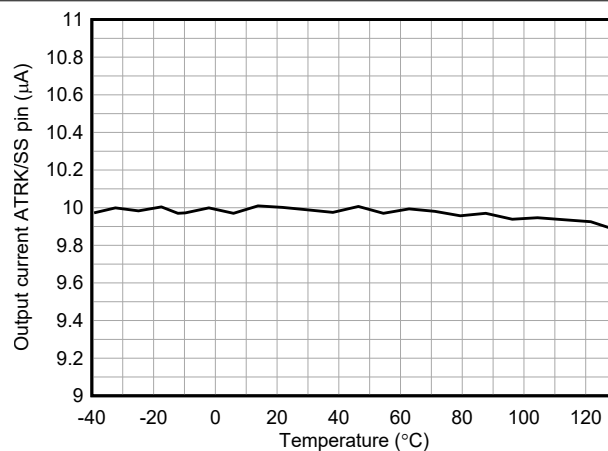
Figure 6-22. Soft-Start current vs Temperature
