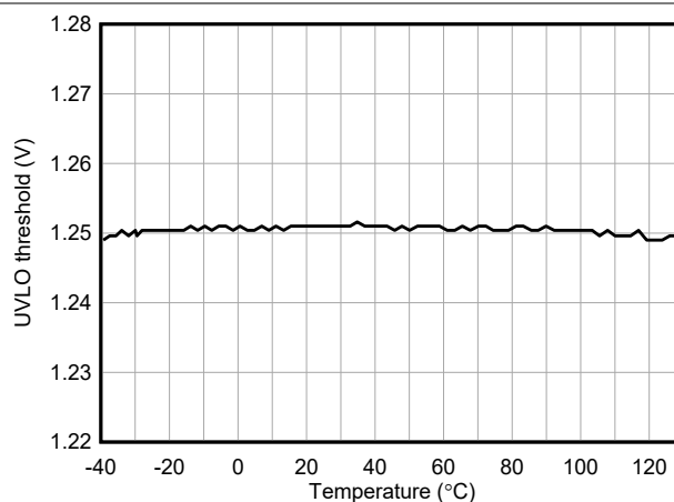
图 6-14. UVLO Threshold Voltage vs Temperature
