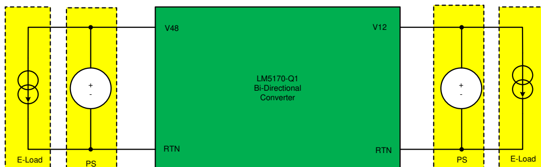
图 10-1. Emulated Dual Battery System With Bench Power Supplies and E-Loads
