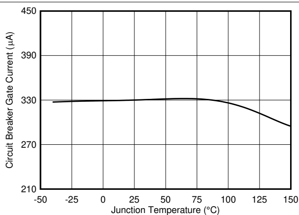
图 7-18. Circuit Breaker Gate Current vs Temperature
