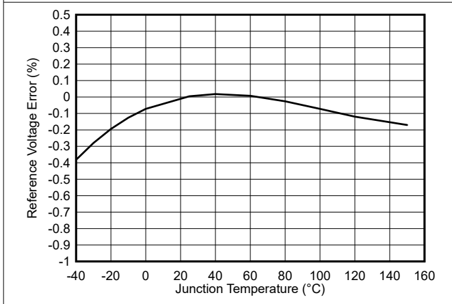
图 7-5. Feedback Comparator Threshold Versus Temperature
