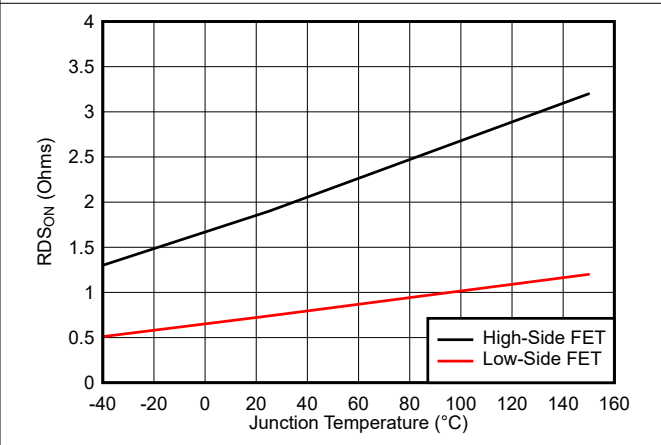
图 7-6. MOSFETs On-State Resistance Versus Temperature
