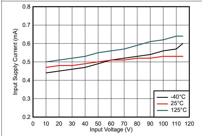
图 7-3. Active Mode Supply Current Versus Input Voltage (FPWM, non-switching)
