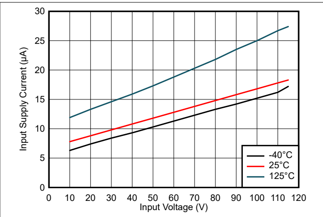
图 7-2. Sleep Mode Supply Current Versus Input Voltage (DEM, non-switching)
