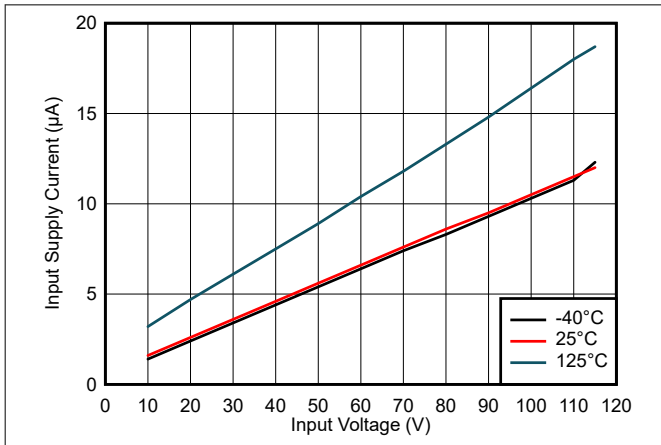
图 7-1. Shutdown Supply Current Versus Input Voltage
