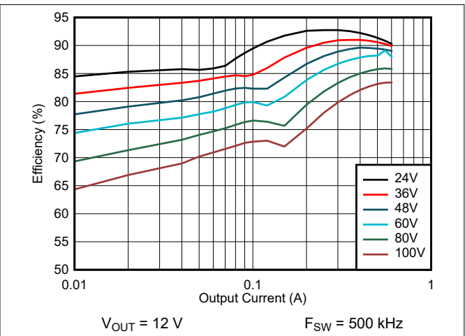
图 9-16. Efficiency: V_{OUT} = 12\text{ V}
