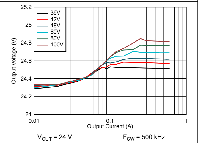
图 9-20. Line and Load Regulation: V_{OUT} = 24\text{ V}
