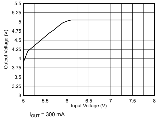
图 8-32. Drop-Out Response
