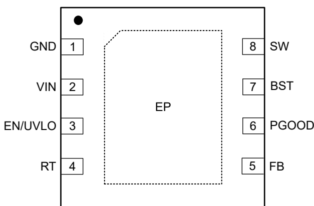
图 5-2. 8-Pin WSON NGU Package (Top View)
