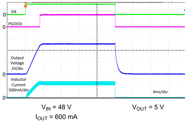
图 8-29. Typical Start-up Waveforms
