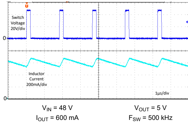
图 8-27. Typical Switching Waveforms
