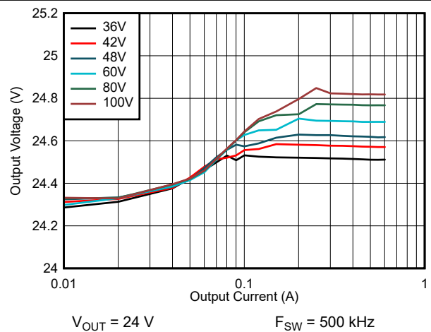
图 8-20. Line and Load Regulation: V_{OUT} = 24\text{ V}
