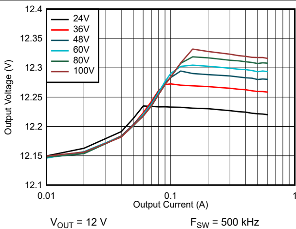
图 8-19. Line and Load Regulation: V_{OUT} = 12\text{ V}
