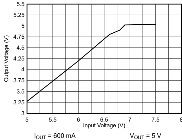
图 8-31. Drop-Out Response
