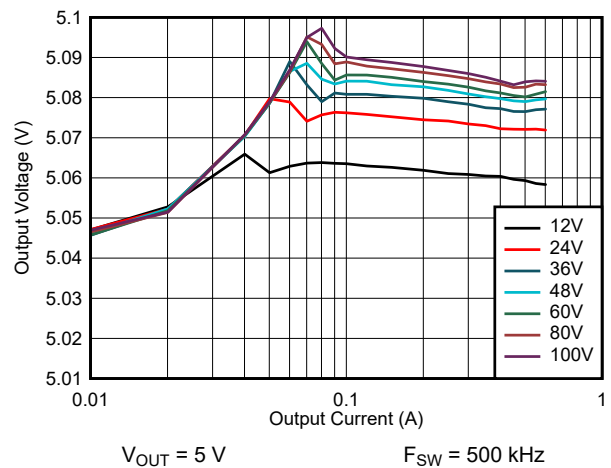
图 8-18. Line and Load Regulation: V_{OUT} = 5\text{ V}
