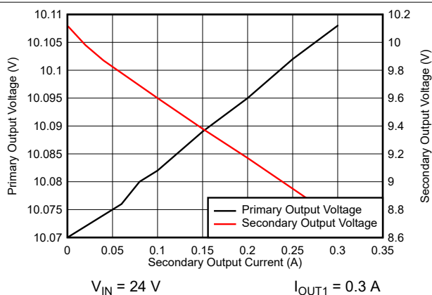
图 8-4. Load Regulation vs Secondary Load Current
