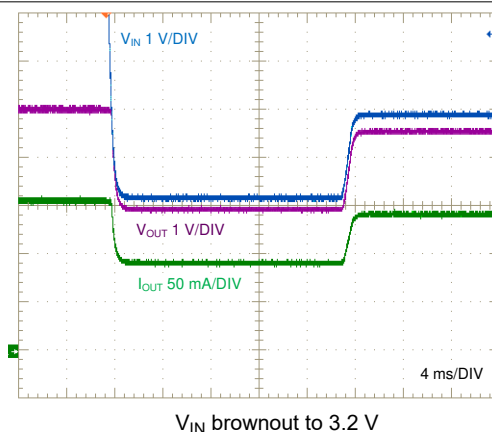
图 8-11. Dropout Performance, 150-mA Resistive Load
