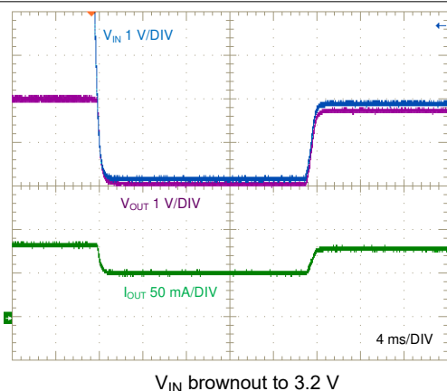
图 8-10. Dropout Performance, 75-mA Resistive Load
