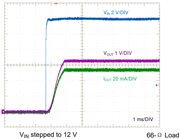
图 8-17. Start-Up, Full Load
