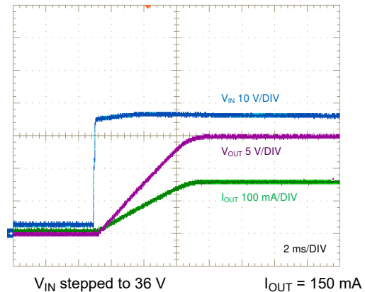
图 8-31. Start-Up, Full Load
