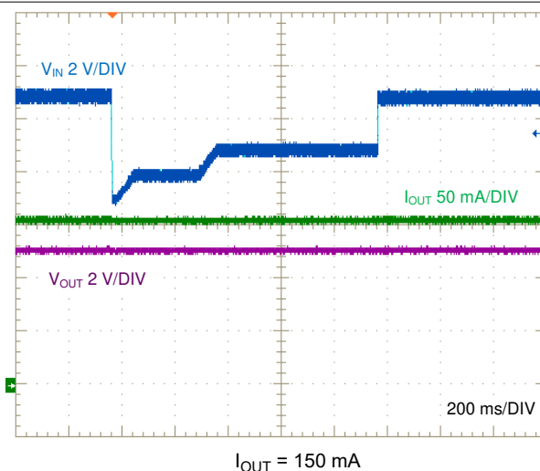
图 8-13. Input Transient (Automotive Cold Crank Profile)
