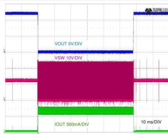
图 8-11. Short Circuit Applied
