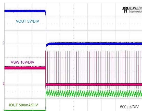
图 8-9. Full-Load Start-up and Shutdown with EN/UVLO
