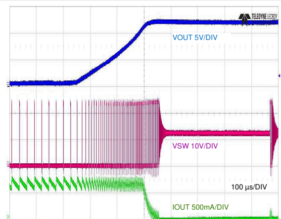
图 8-10. Pre-bias Start-up with EN/UVLO
