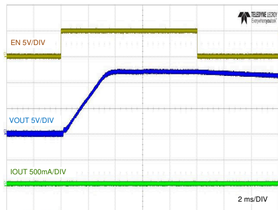
图 8-8. No-Load Start-up and Shutdown with EN/UVLO
