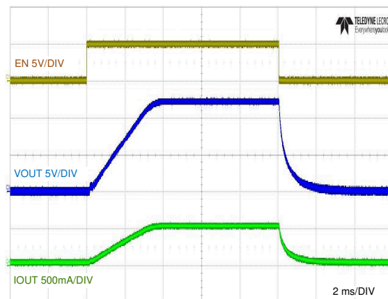
图 8-9. Full-Load Start-up and Shutdown with EN/UVLO
