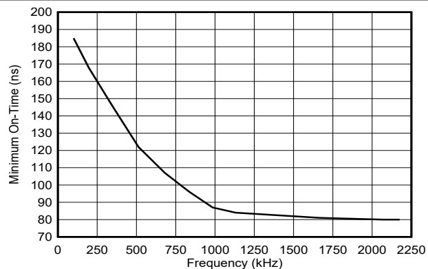
图 8-15. Minimum On Time vs Frequency
