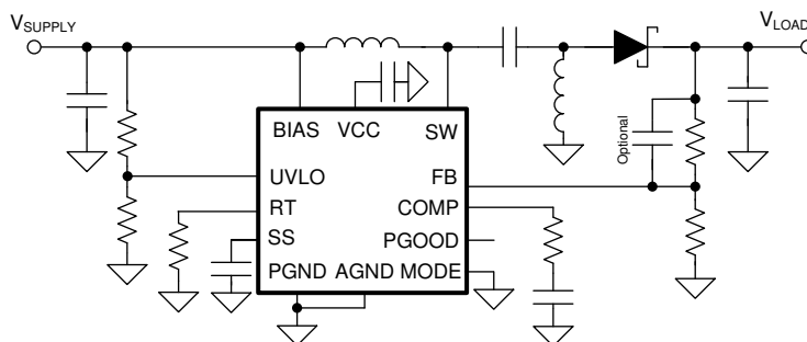
图 10-4. Typical SEPIC Application
