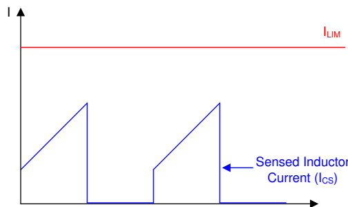
图 8-19. Current Sensing (b) at Current Limit Comparator Inputs
