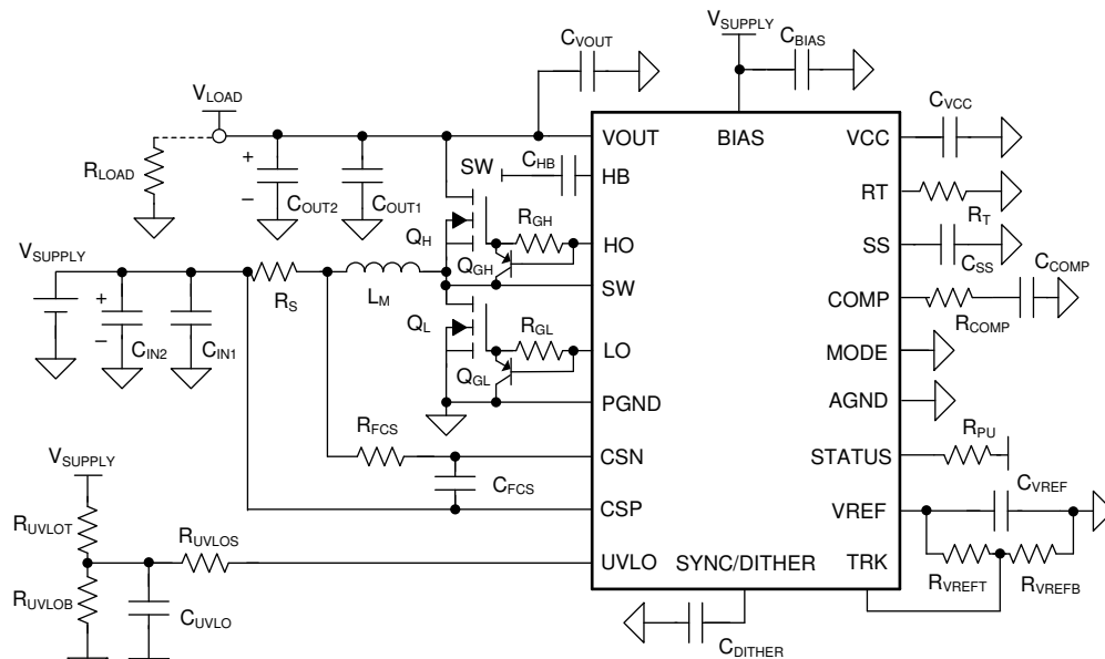
图 10-1. Typical Synchronous Boost Converter with Optional Components
