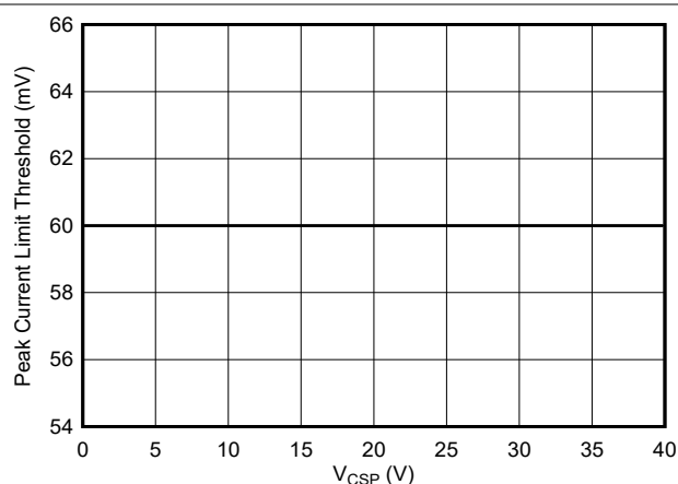
图 8-11. Peak Current Limit Threshold vs V_{CSP}
