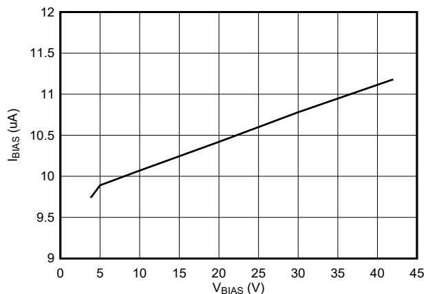
图 8-6. VBIAS vs IBIAS (Bypass Mode, Charge Pump Off)
