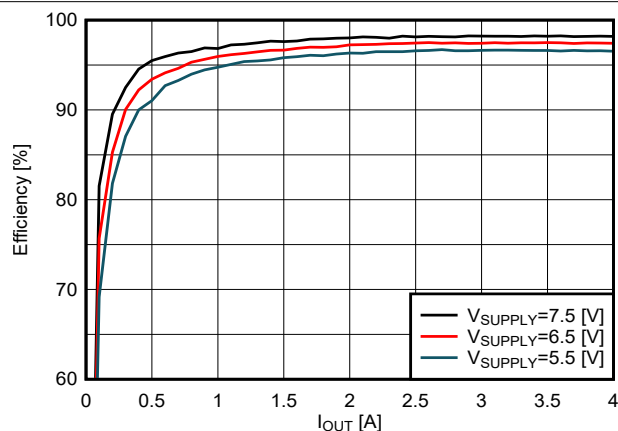
图 10-4. Efficiency vs. I_{OUT} , V_{OUT} = 8.5 V (FPWM)
