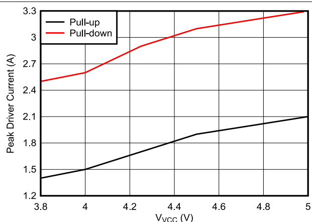
图 8-10. V_{VCC} vs Peak Driver Current
