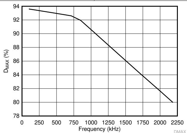
图 8-17. D_{MAX} vs Frequency
