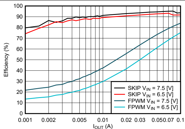
图 10-5. Efficiency vs. I_{OUT} , V_{OUT} = 8.5 -V Light Load
