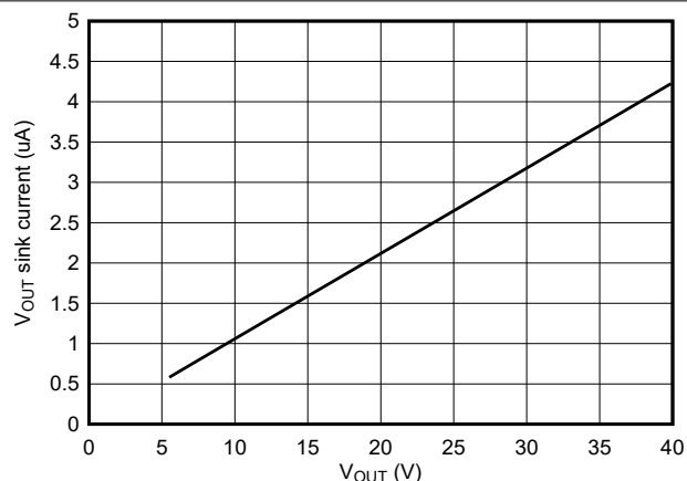
图 8-14. V_{OUT} Sink Current vs V_{OUT} (Deep Sleep)
