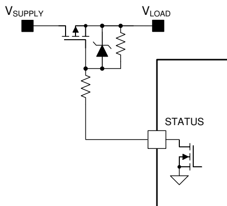
图 9-1. Bypass Switch Control Example
