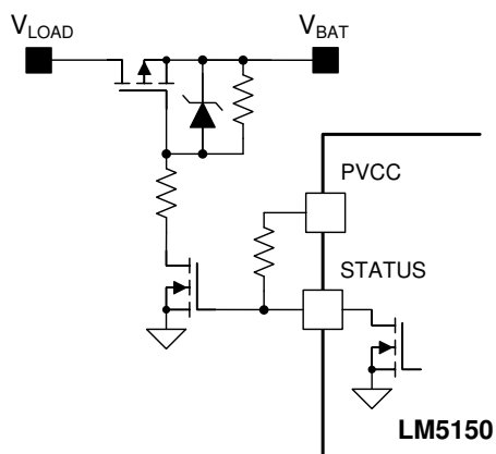
图 9-2. Disconnection Switch Control Example
