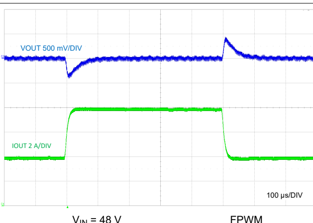
图 9-28. Load Transient, 4 A to 8 A
