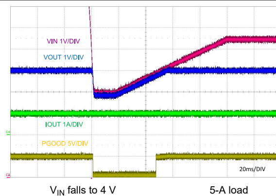
图 9-11. Cold-Crank Response to V_{IN} = 4 V
