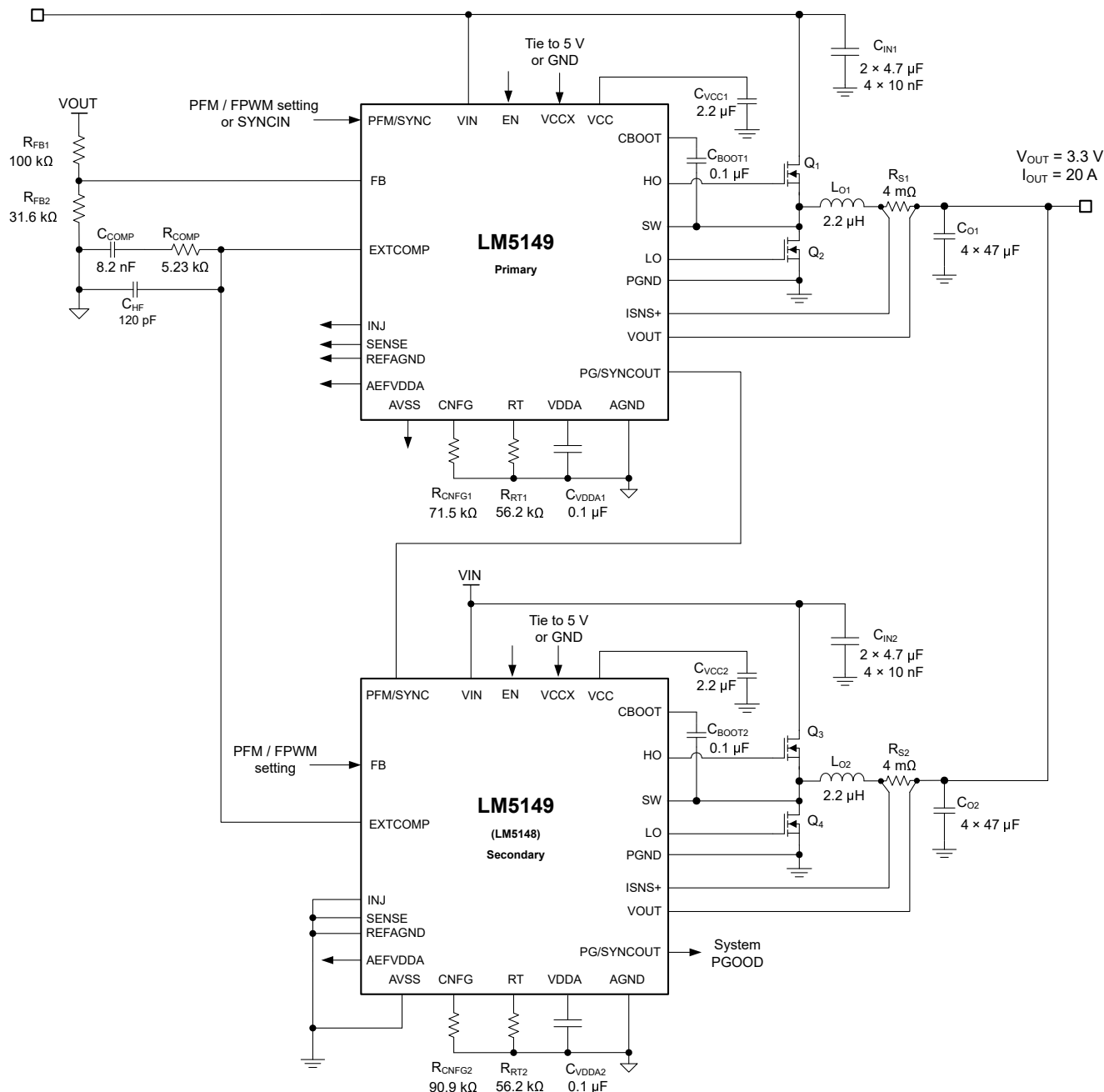
图 9-40. Application Circuit 4 With Two LM5149 Buck Controllers at 400 kHz
