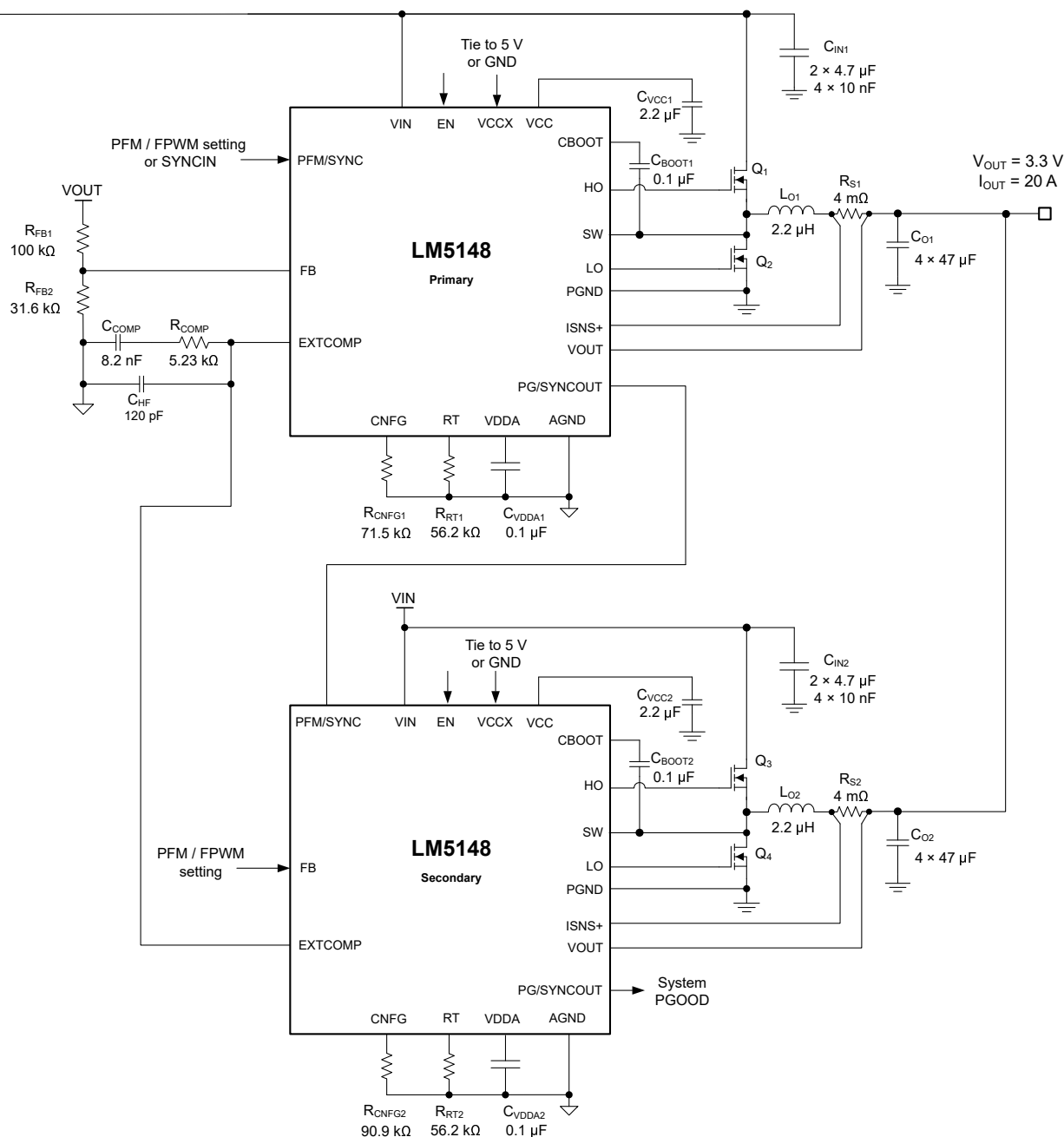
图 9-39. Application Circuit 4 with Two LM5148 Buck Regulators Switching at 400 kHz
