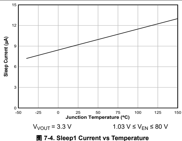
图 7-4. Sleep1 Current vs Temperature
