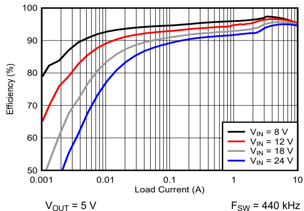
图 7-2. Efficiency vs Load, Log Scale
