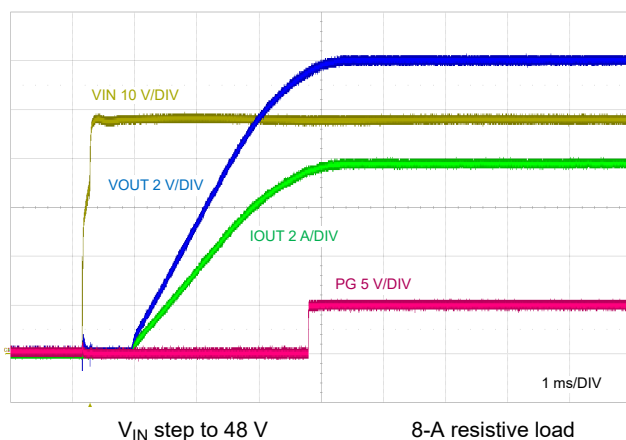
图 9-22. Start-Up Characteristic
