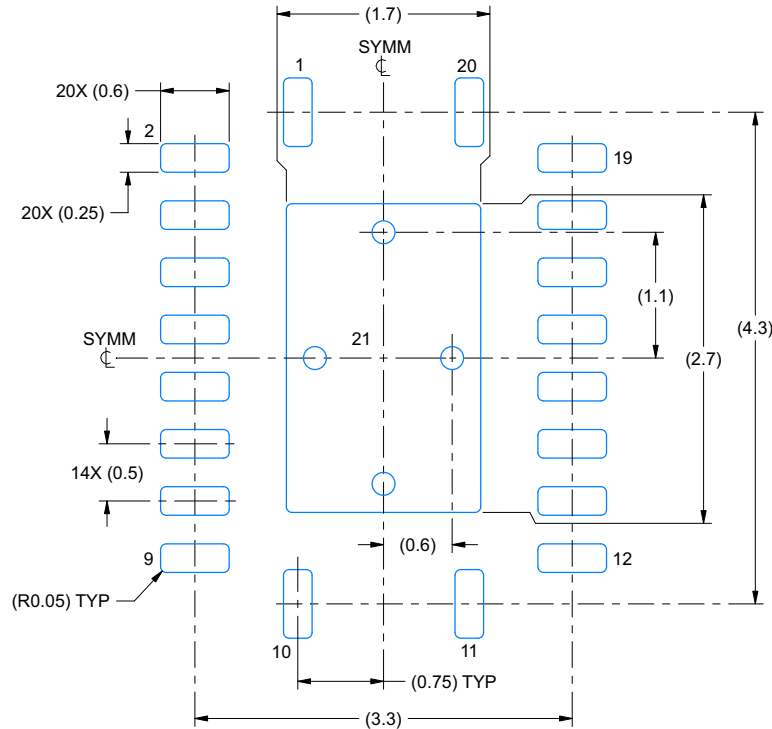
LAND PATTERN EXAMPLE EXPOSED METAL SHOWN SCALE:18X
