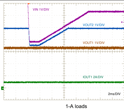
图 9-10. Cold-Crank Response to V_{IN} = 3.8\text{ V}
