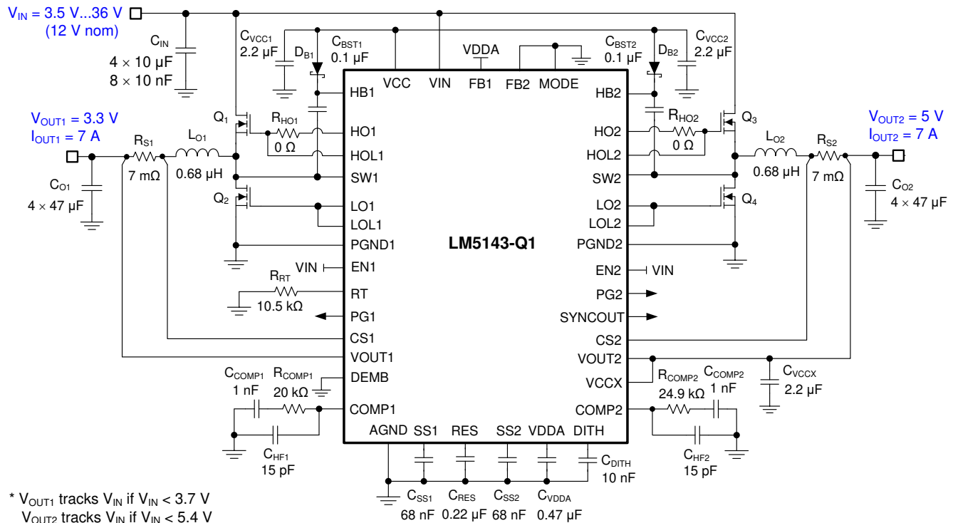
图 9-4. Application Circuit 1 With LM5143-Q1 Buck Regulator at 2.1 MHz
