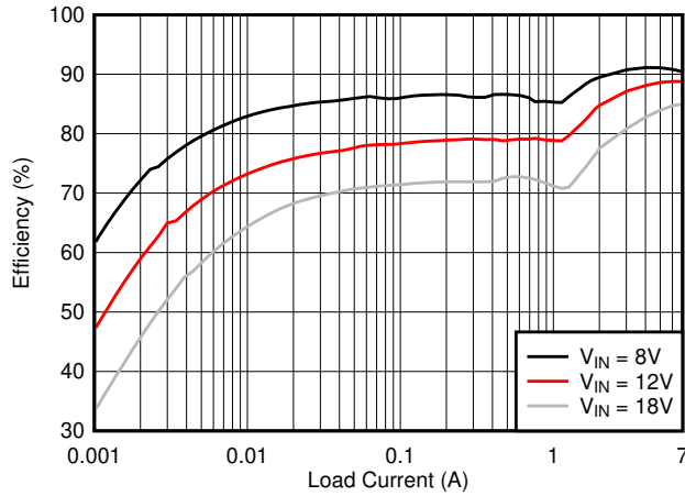
图 9-5. Efficiency versus I_{OUT}
