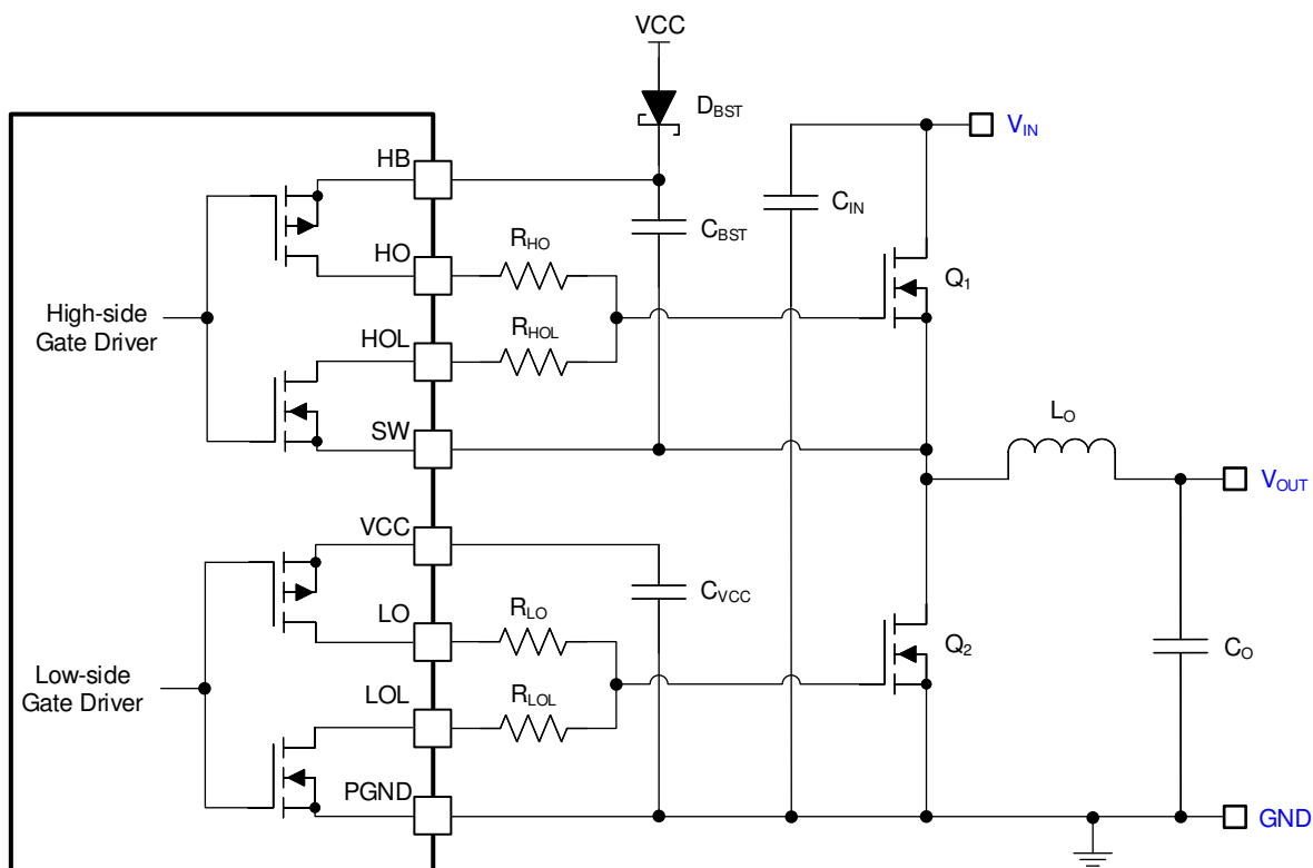
图 8-7. Integrated MOSFET Gate Drivers
