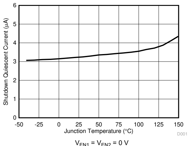
图 7-6. Shutdown Current versus Temperature
