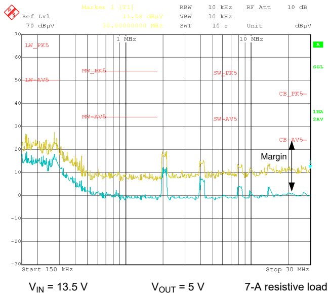
图 9-19. CISPR 25 Class 5 Conducted EMI, 150 kHz to 30 MHz
