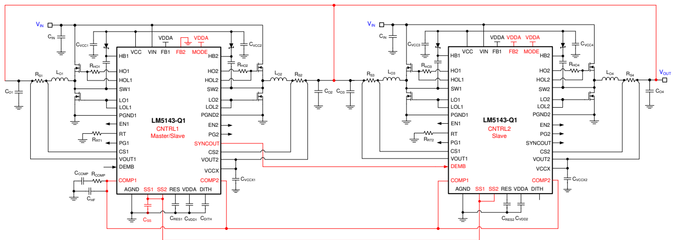
8-10. Multiphase Regulator Schematic Configured for Single-Output Interleaved Operation
