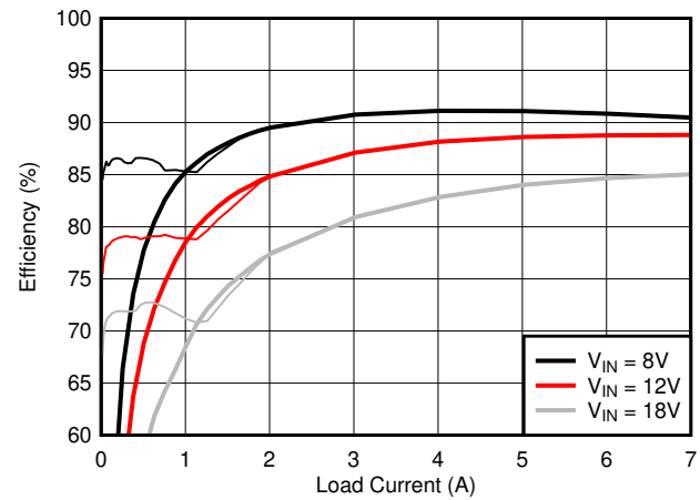
图 9-6. Efficiency versus I_{OUT}
