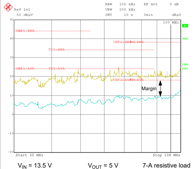
图 9-20. CISPR 25 Class 5 Conducted EMI, 30 MHz to 108 MHz
