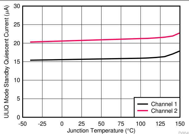
图 7-9. ULIQ Mode Standby Current versus Temperature
