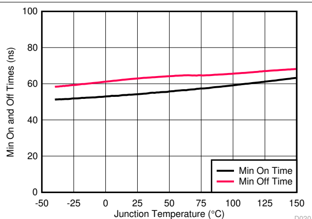
图 7-24. Minimum On Time and Off Time (HO1) versus Temperature
