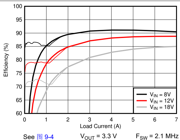
图 7-2. Efficiency versus Load
