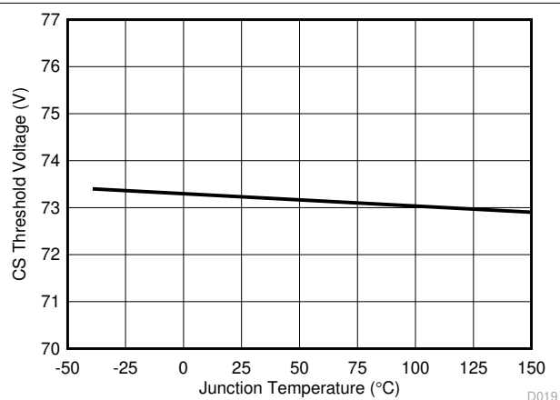
图 7-22. Current Sense (CS1) Threshold versus Temperature
