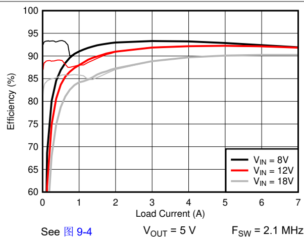
图 7-1. Efficiency versus Load
