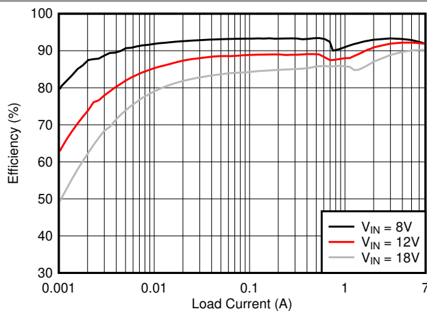
图 9-7. Efficiency versus I_{OUT} , Log Scale
