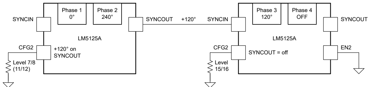
Figure 6-6. 3-Phase Configuration
