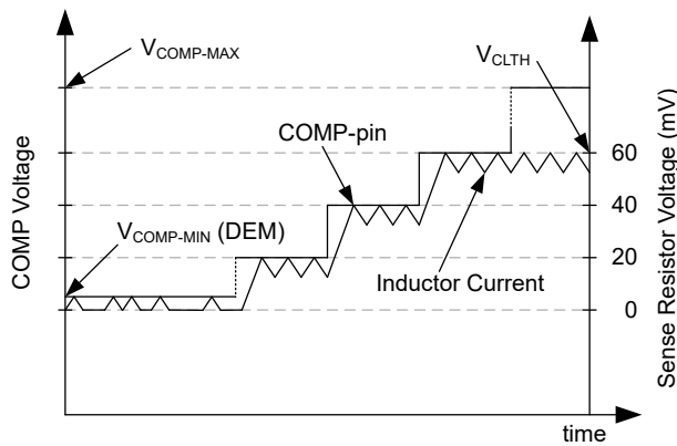
Figure 6-21. COMP-pin and Sense Resistor Voltage limiting the switch current (DEM)
