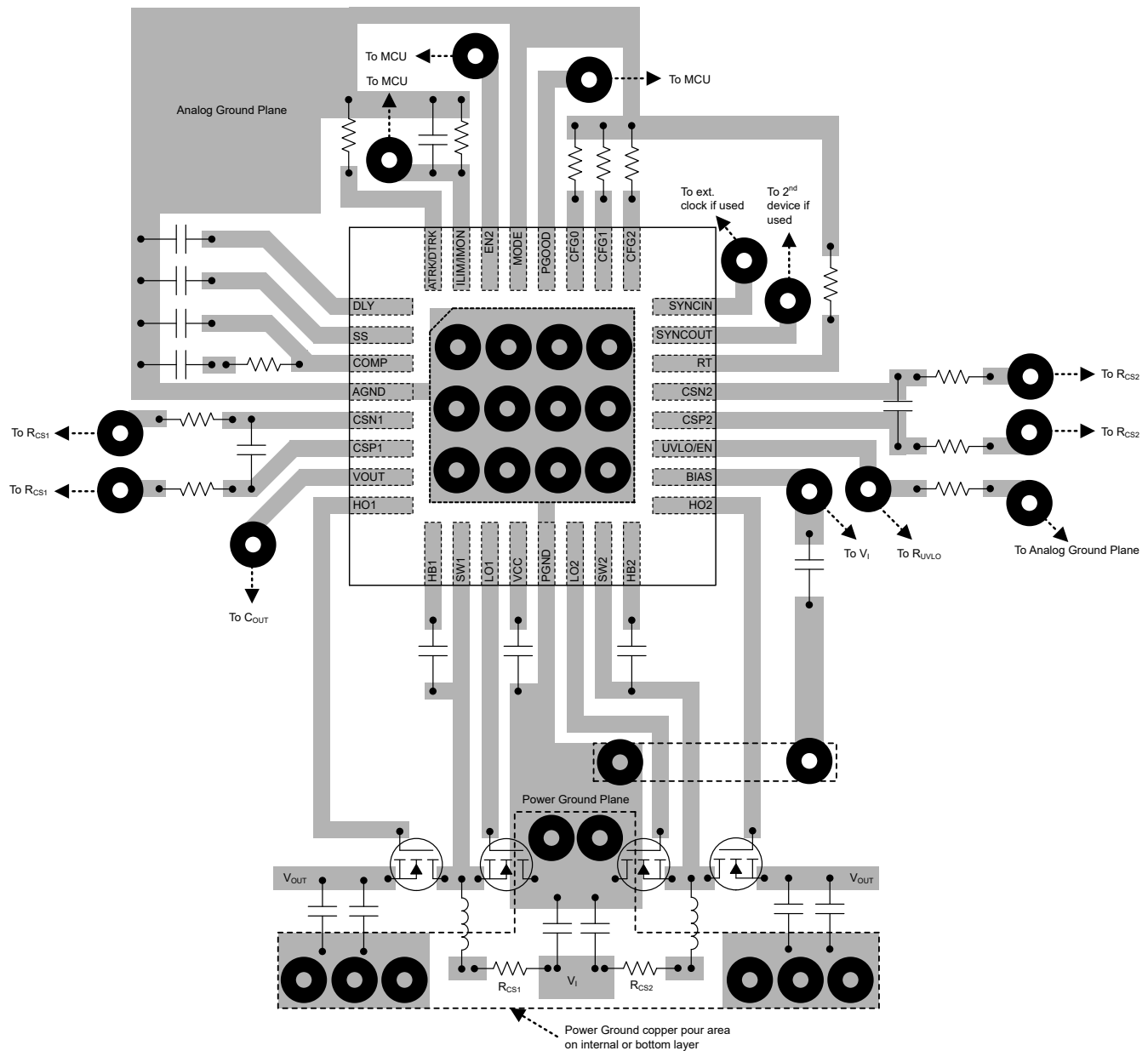
Figure 7-22. Layout Example
