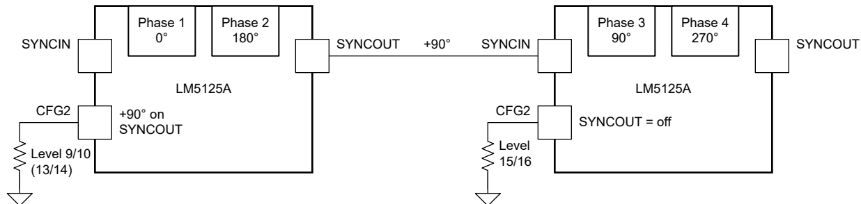
Figure 6-7. 4-Phase Configuration
