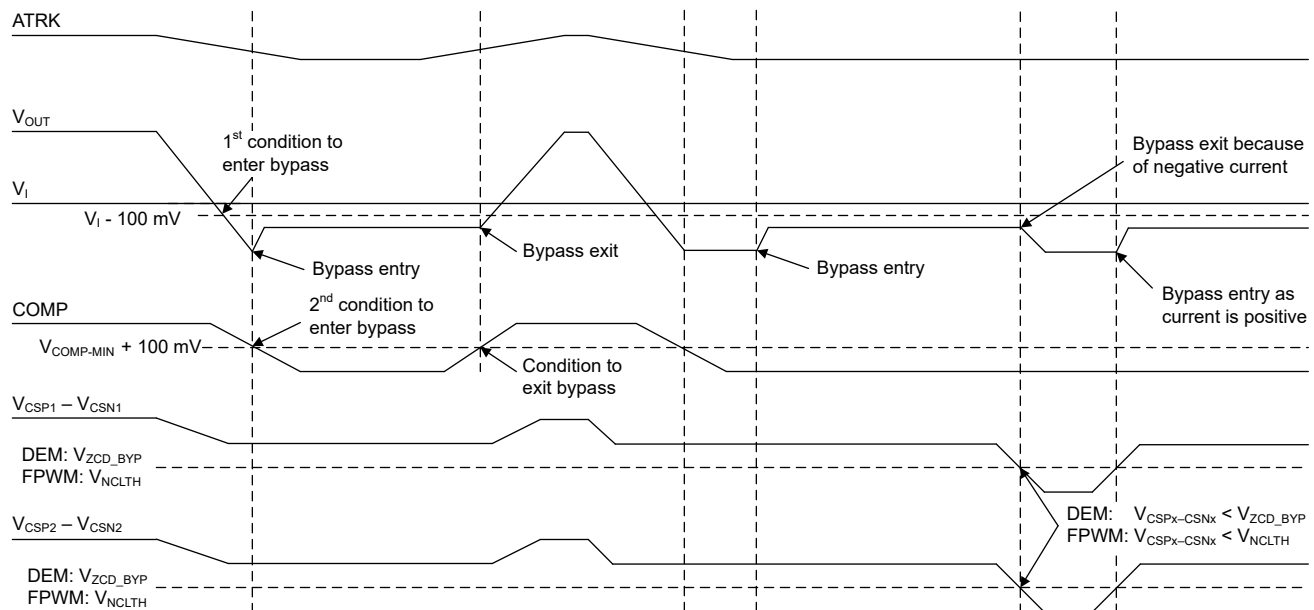
Figure 6-12. Bypass Mode Entry, Exit
