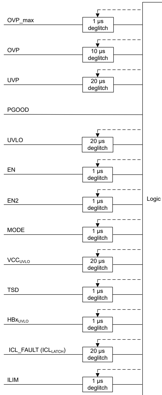
Figure 6-25. Signal Deglitching
