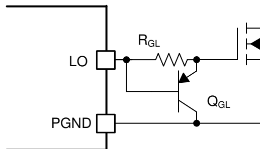
Figure 6-26. Slew Rate Control
