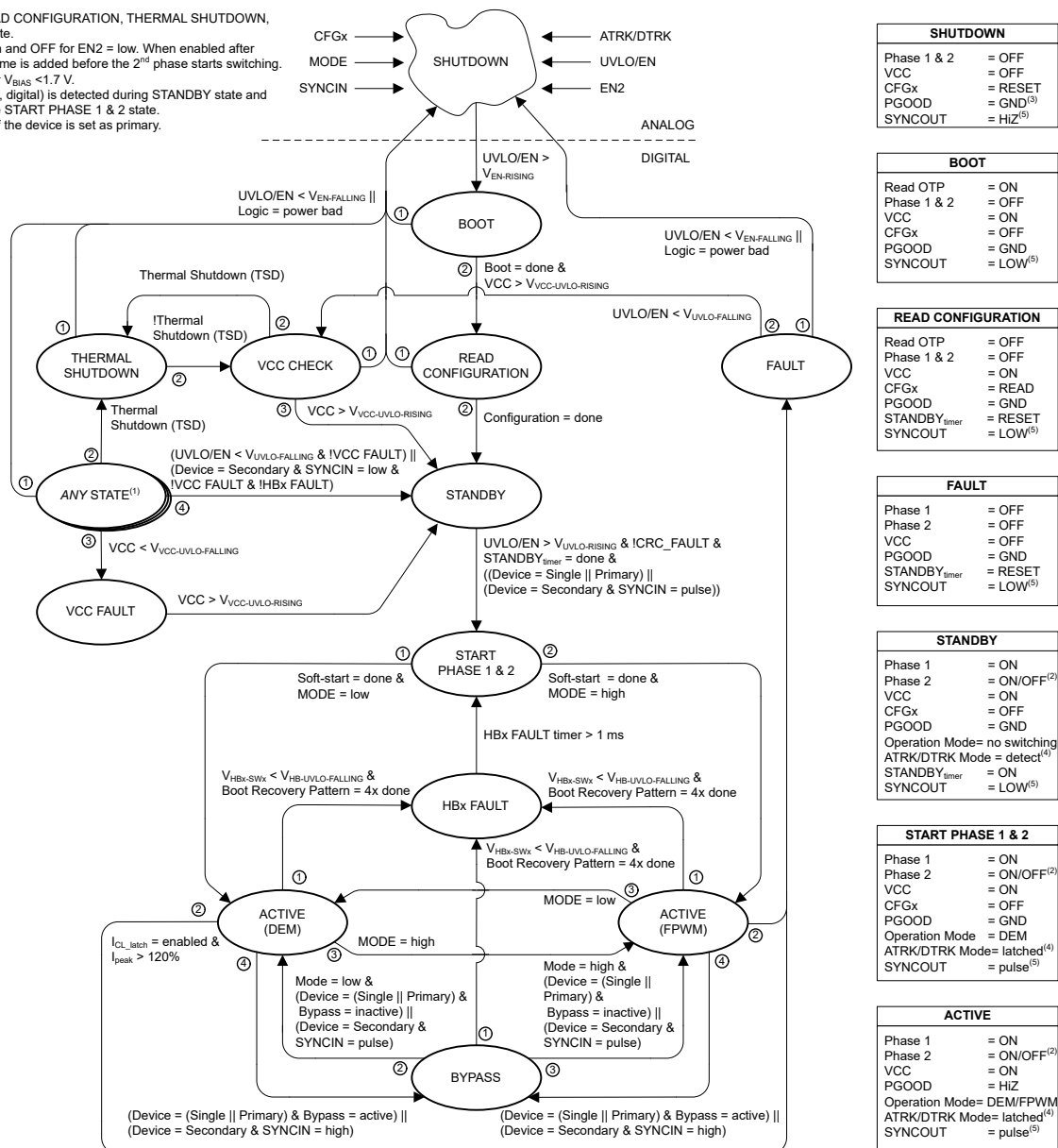
Figure 6-27. Functional State Diagram
