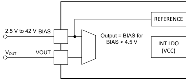
Figure 6-13. On the Fly BIAS Supply Selection
