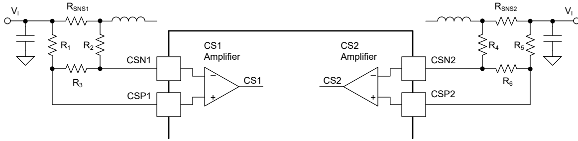
Figure 6-20. Peak Limit adjustment through additional resistors
