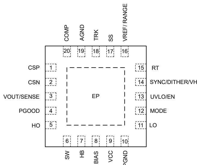
图 5-1. 20-Pin QFN with Wettable Flanks RGR Package (Top View)
