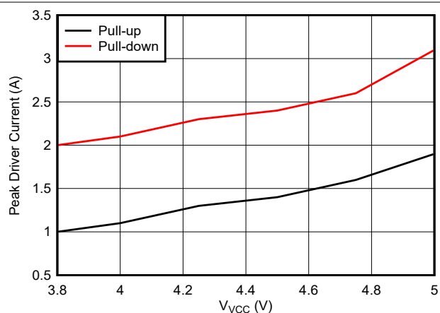
图 6-16. V_{CC} vs Peak Driver Current
