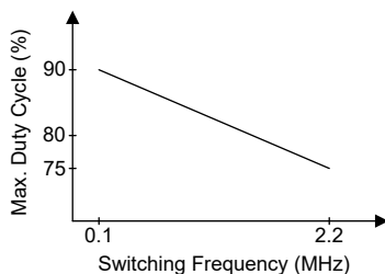
图 7-17. Switching Frequency vs max. Duty Cycle
