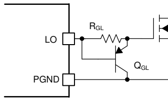
图 7-19. Slew Rate Control
