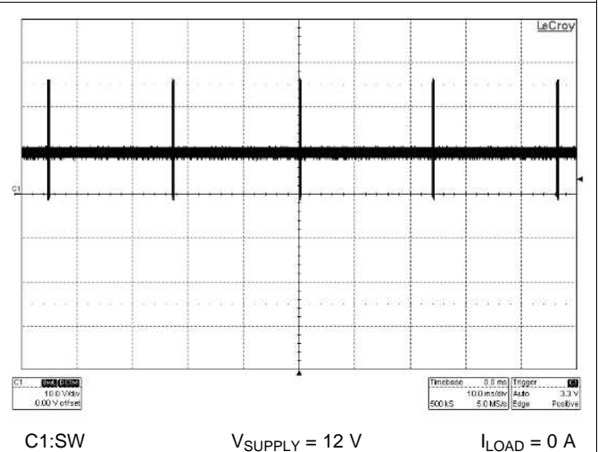
Figure 46. Skip Cycle
