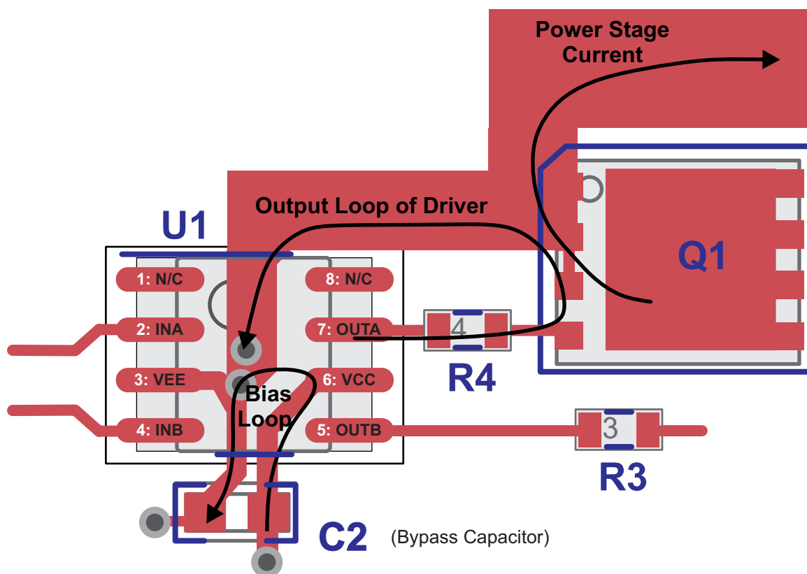
Figure 15. Layout
