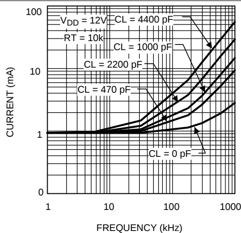
Figure 1. I_{DD} vs Frequency
