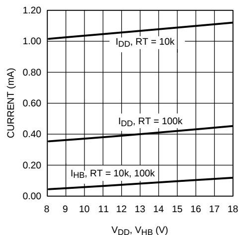
Figure 3. Quiescent Current vs Supply Voltage
