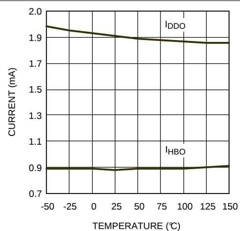
Figure 2. Operating Current vs Temperature
