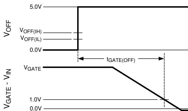
Figure 2. Gate OFF Timing for OFF Pin Low to High Transition
